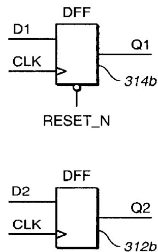
c. Implementation created by AMBIT BuildGates
