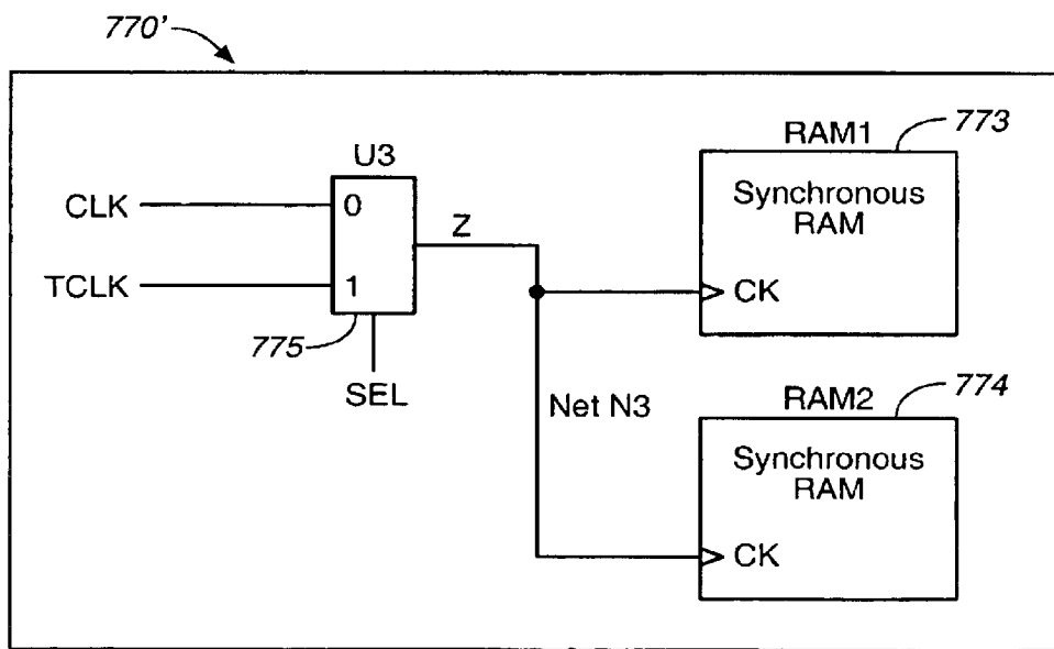
(b) After initial mapping
