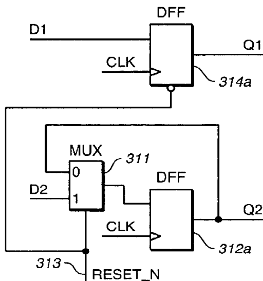
b. Implementation created by Synopsys Design Compiler
