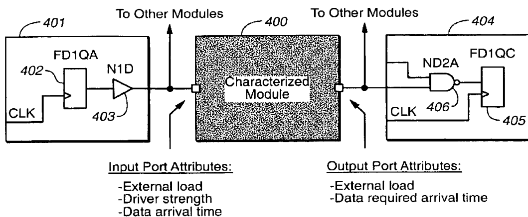
FIG._15 :Characterization.
