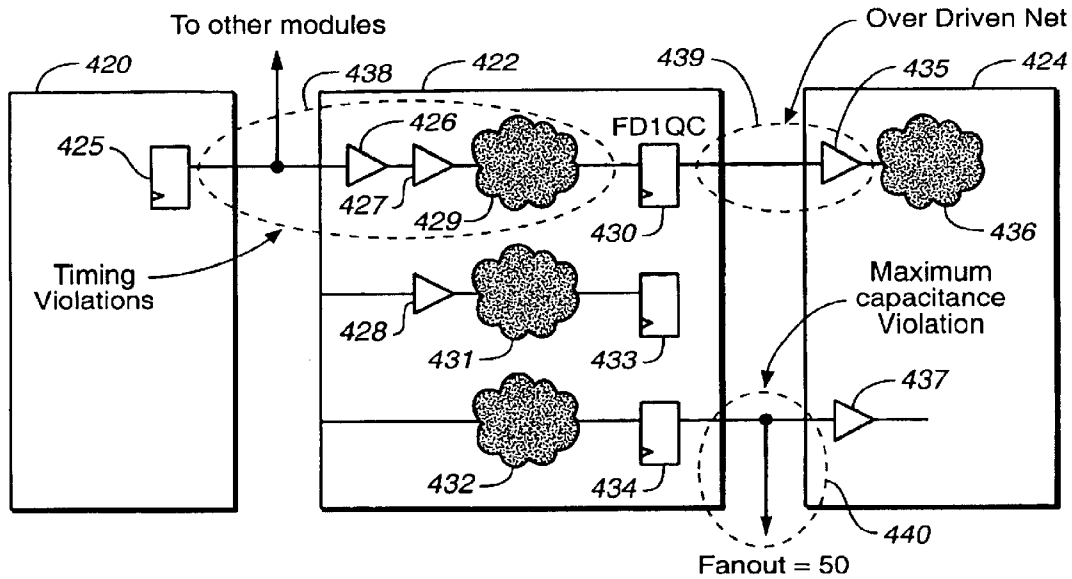
FIG. 18 : Results after initial mapping.
