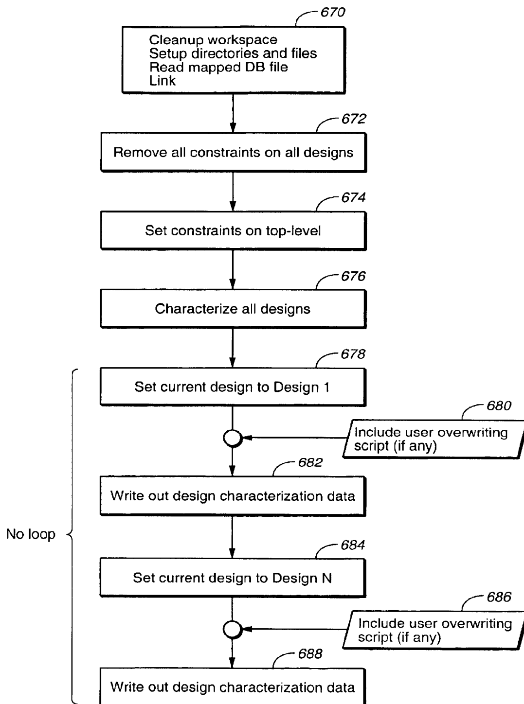
FIG. 30 : Structure of characterization script
