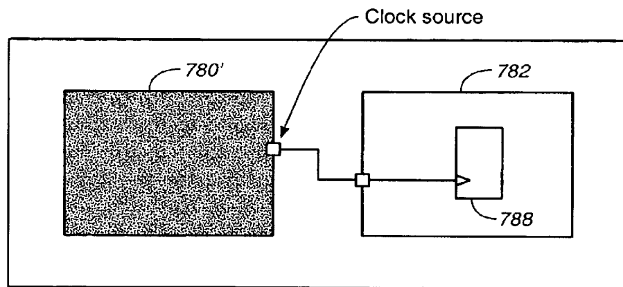
(a) After making the clock generator a blackbox for VEGA analysis
