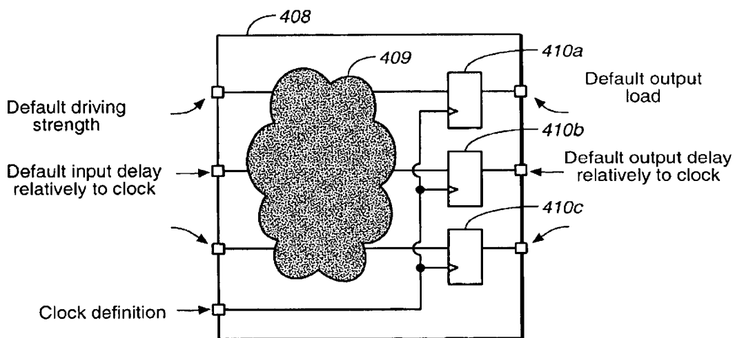
FIG._17 :Default constraints used for initial mapping.
