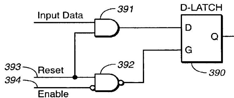
FIG._37 : Failing implementation of a latch with clear.
