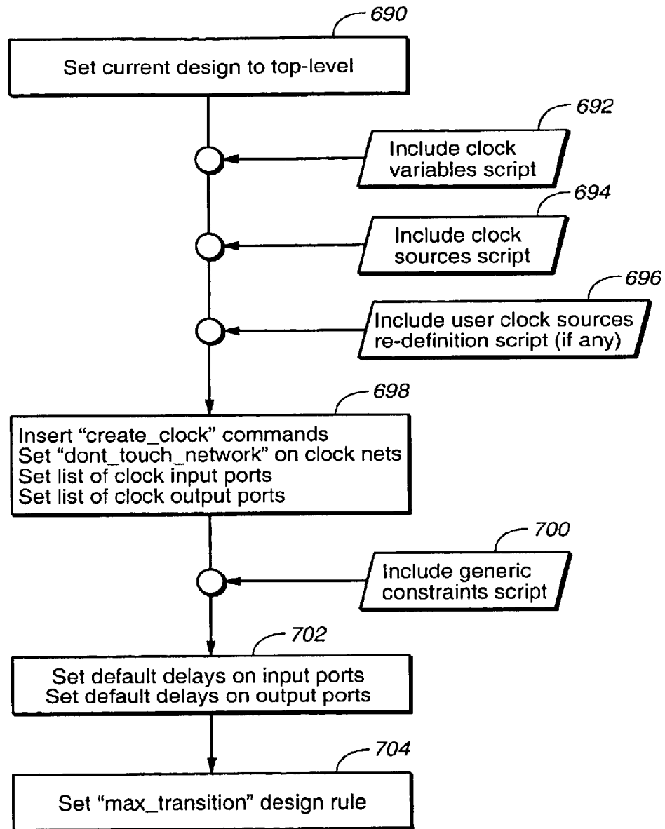
FIG. 31 : Structure of constraints setting on top-level
