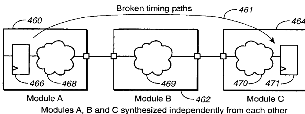
FIG._20A : Broken timing paths
