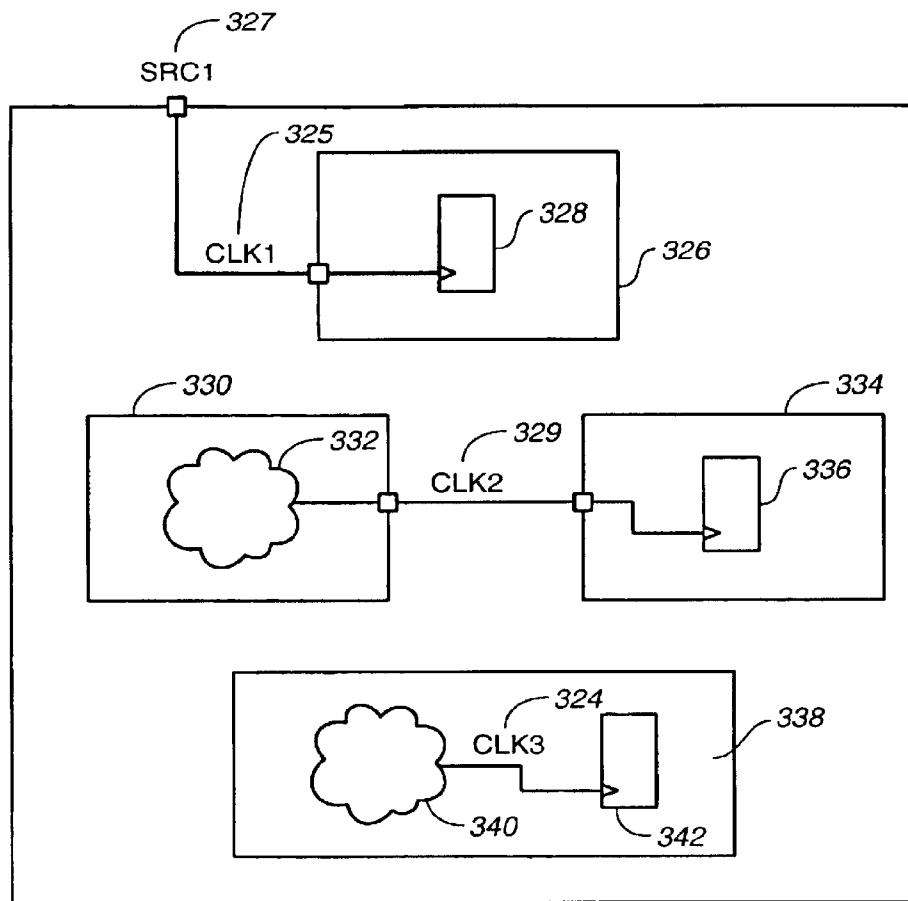
FIG. 39 : External and internal clocks.
