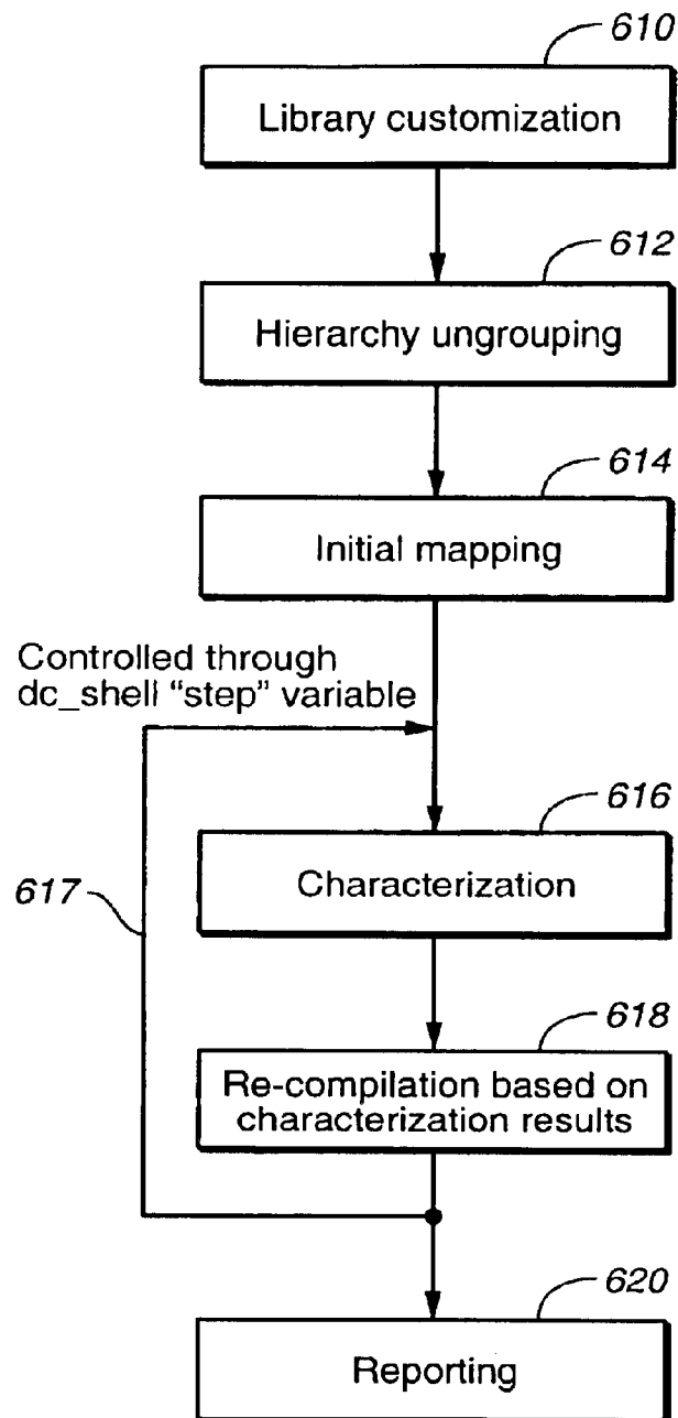
FIG. 27 : Script flow implemented by VEGA
