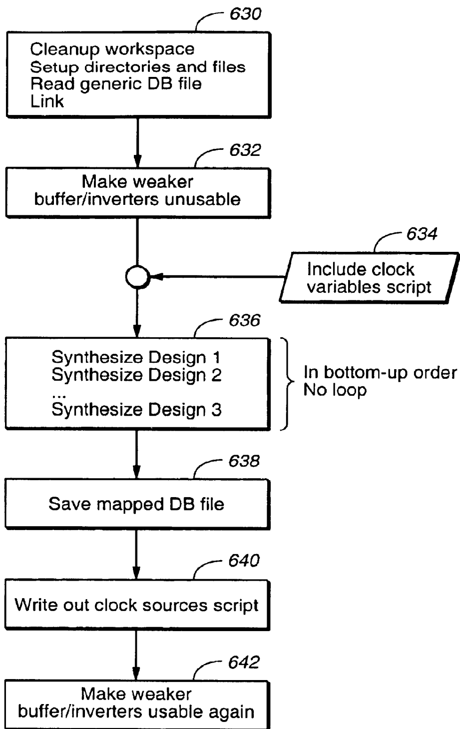
FIG. 28 : Structure of initial mapping script
