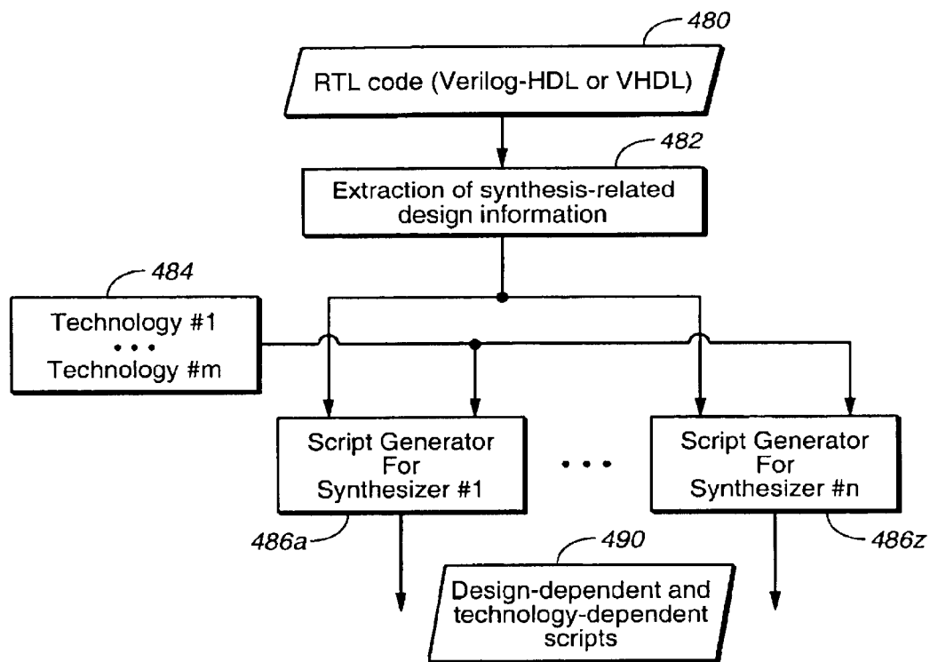
FIG. 21 : Automatic Script Generation
