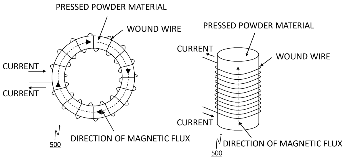
EXEMPLARY CONCEPTUAL DIAGRAM OF RING-SHAPED INDUCTOR
