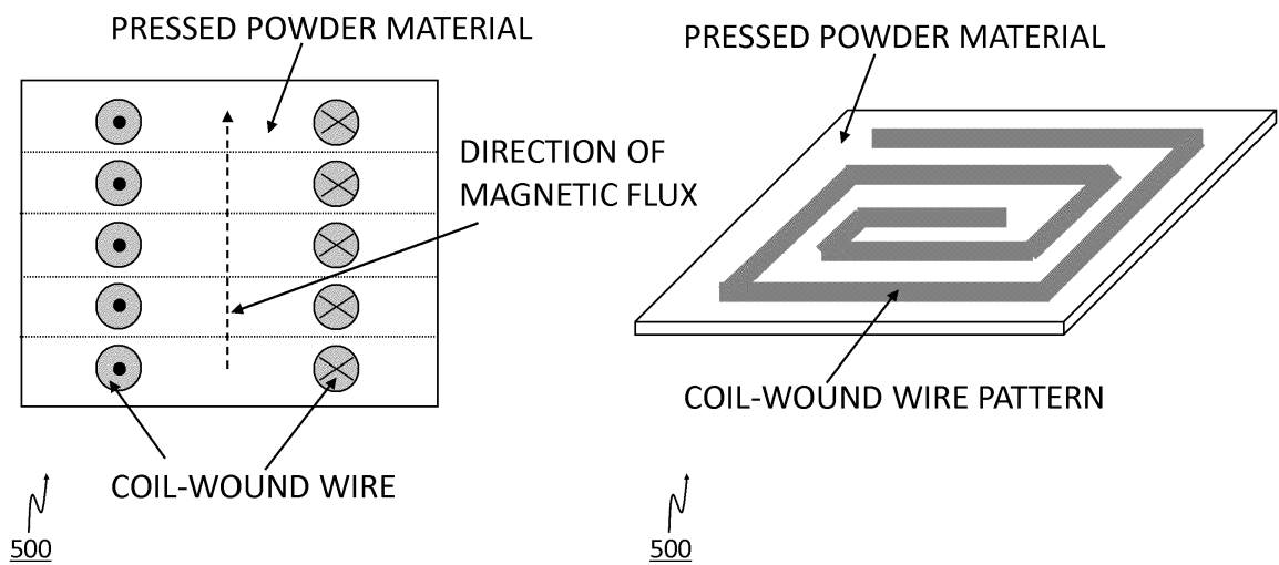
EXEMPLARY CONCEPTUAL CROSS-SECTIONAL VIEW OF CHIP INDUCTOR
