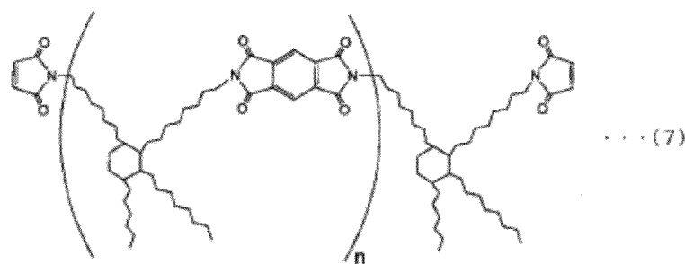
[Chemical formula 6]
