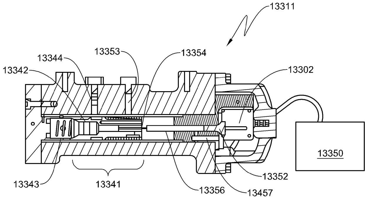
SECTION B-B FIG. 65B
