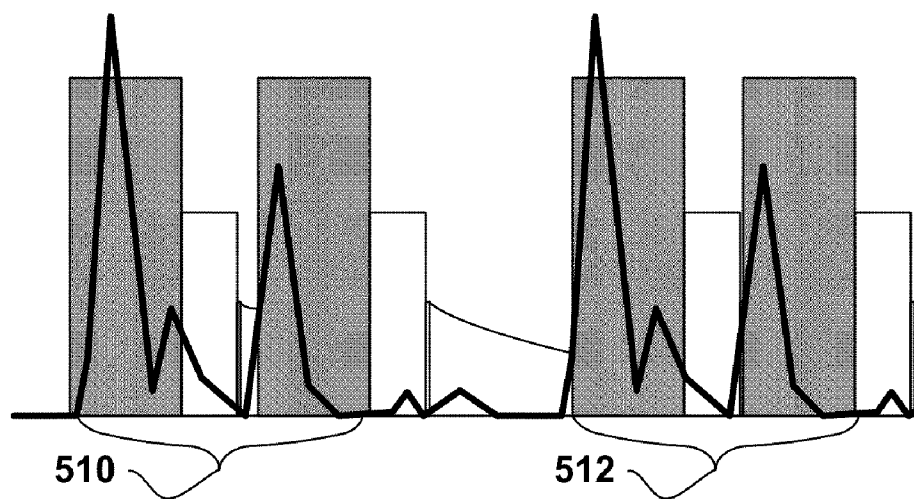
Overdetecting T-Waves
