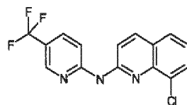
Formula (Ia)
