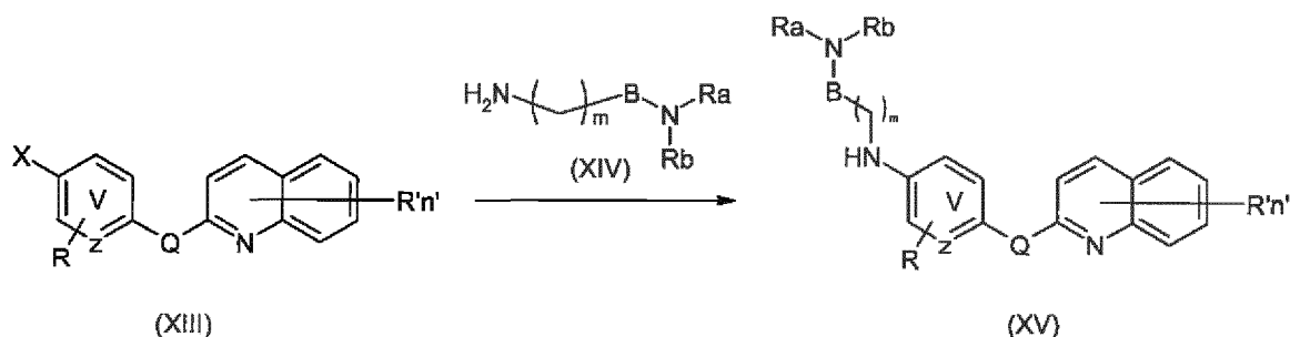
Scheme 4
