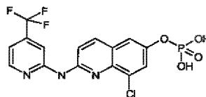
Formula (Ib)
