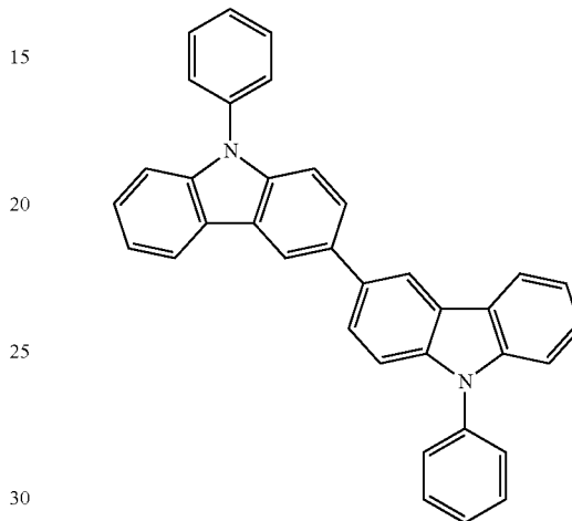
PCCP
