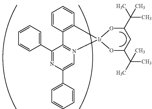
[Ir(tppr) 2 (dpm)]
