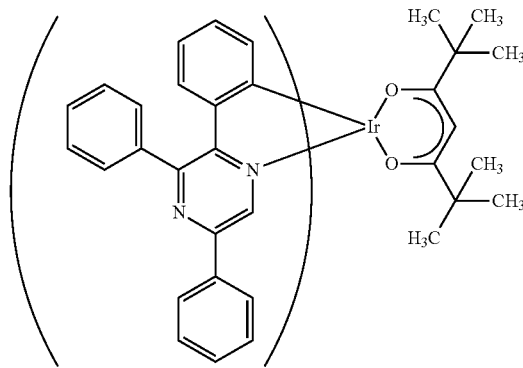
[\text{Ir}(\text{tppr})_2(\text{dpm})]
