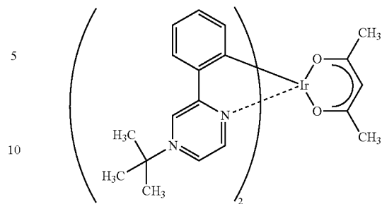
[Ir(tBuppm) 2 (acac)]
