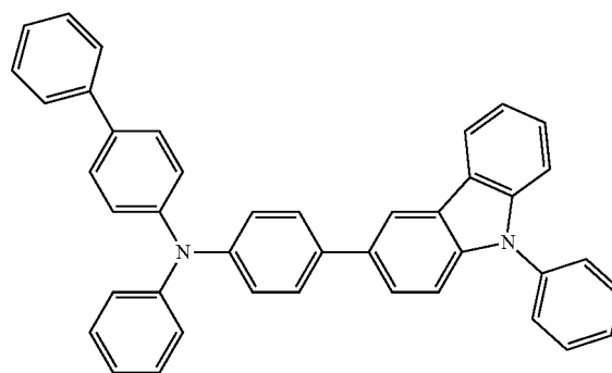
PCBA1BP
