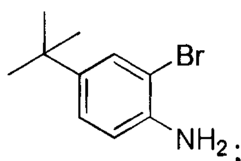
2-bromo-4- tert -butylaniline
