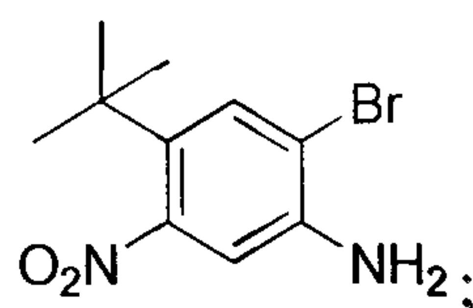
2-bromo-4- tert -butyl-5-nitroaniline
