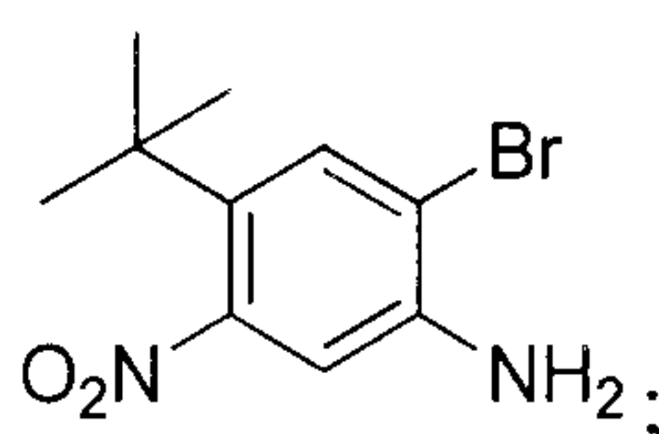
2-bromo-4- tert -butyl-5-nitroaniline
