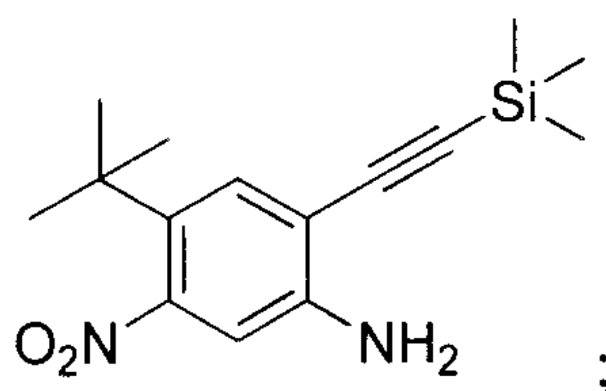
4- tert -butyl-5-nitro-2-((trimethylsilyl)ethynyl)aniline
