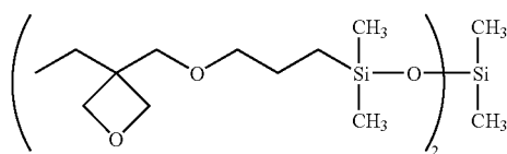
Exemplary Compound 2
