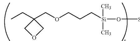
Exemplary compound 3
