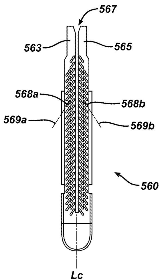
FIG. 14 PRIOR ART
