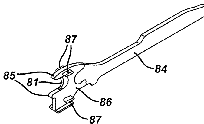
FIG. 5 PRIOR ART
