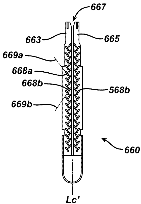
FIG. 15 PRIOR ART
