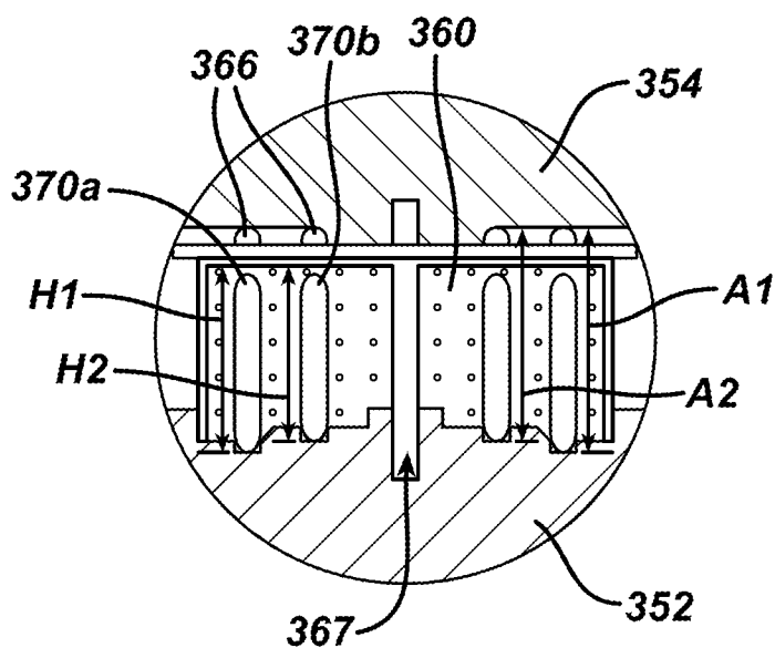
FIG. 11 PRIOR ART
