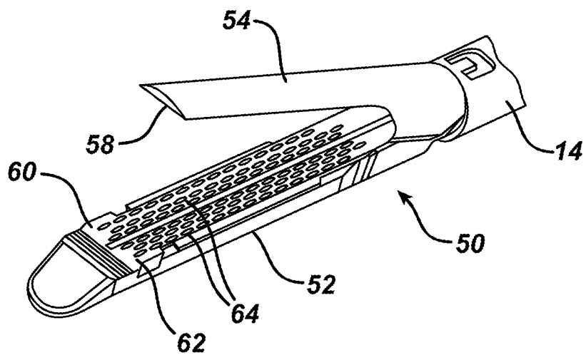
FIG. 8 PRIOR ART
