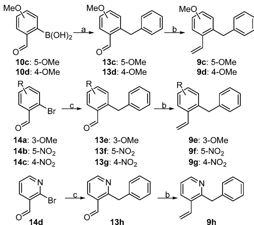
Scheme 2: Synthesis of 16-24
