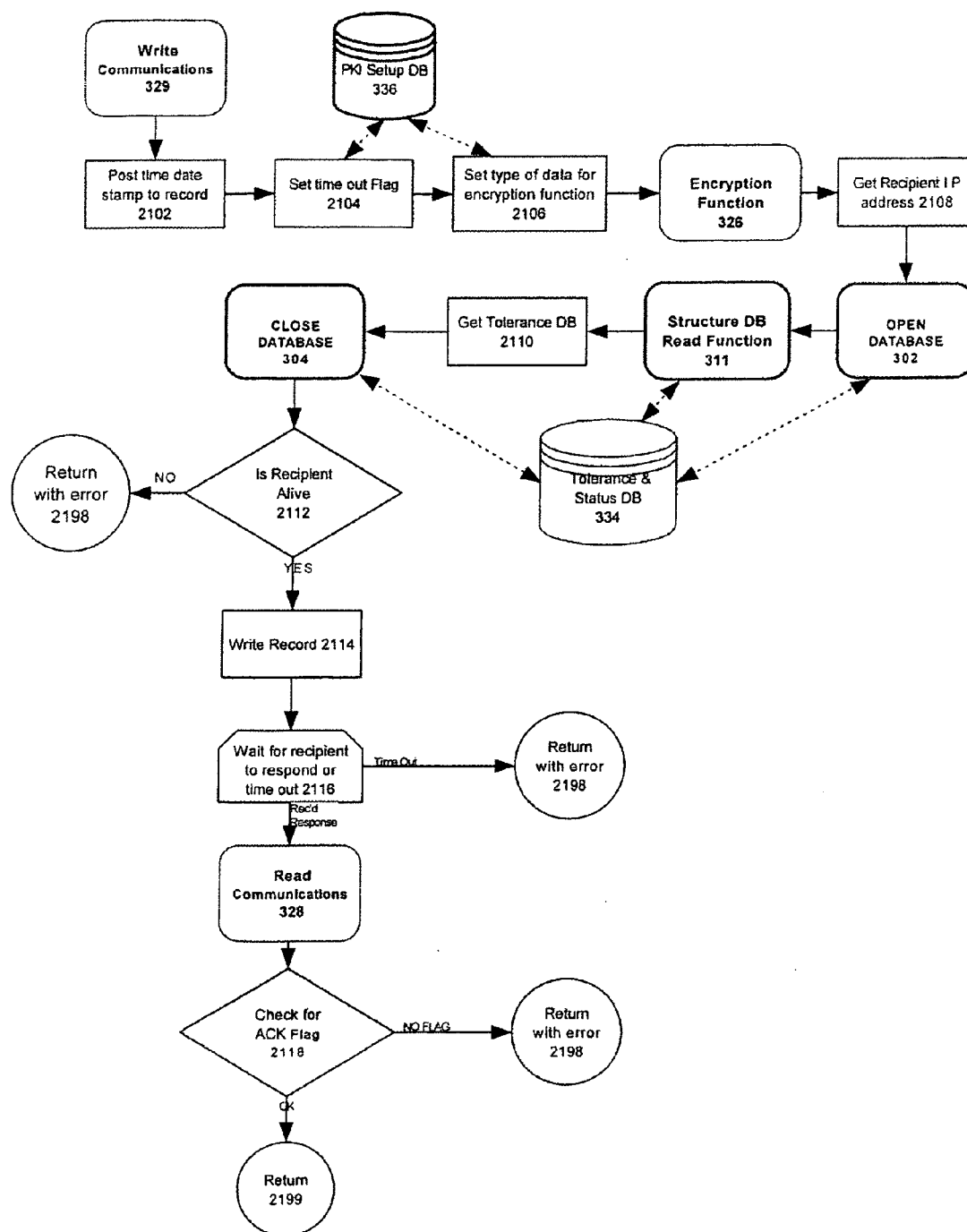
FIGURE 21 ITEM 329
