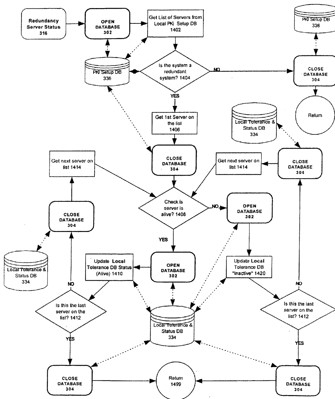
FIGURE 14 ITEM 316
