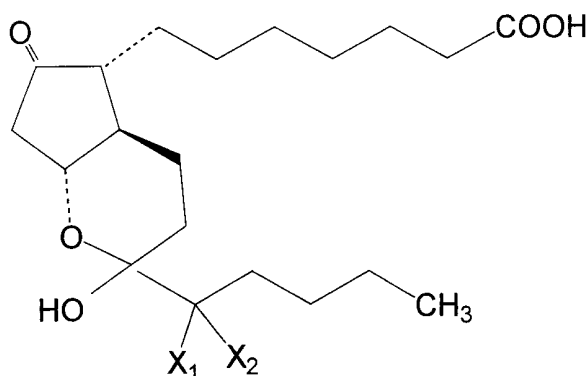
Tautomer II
