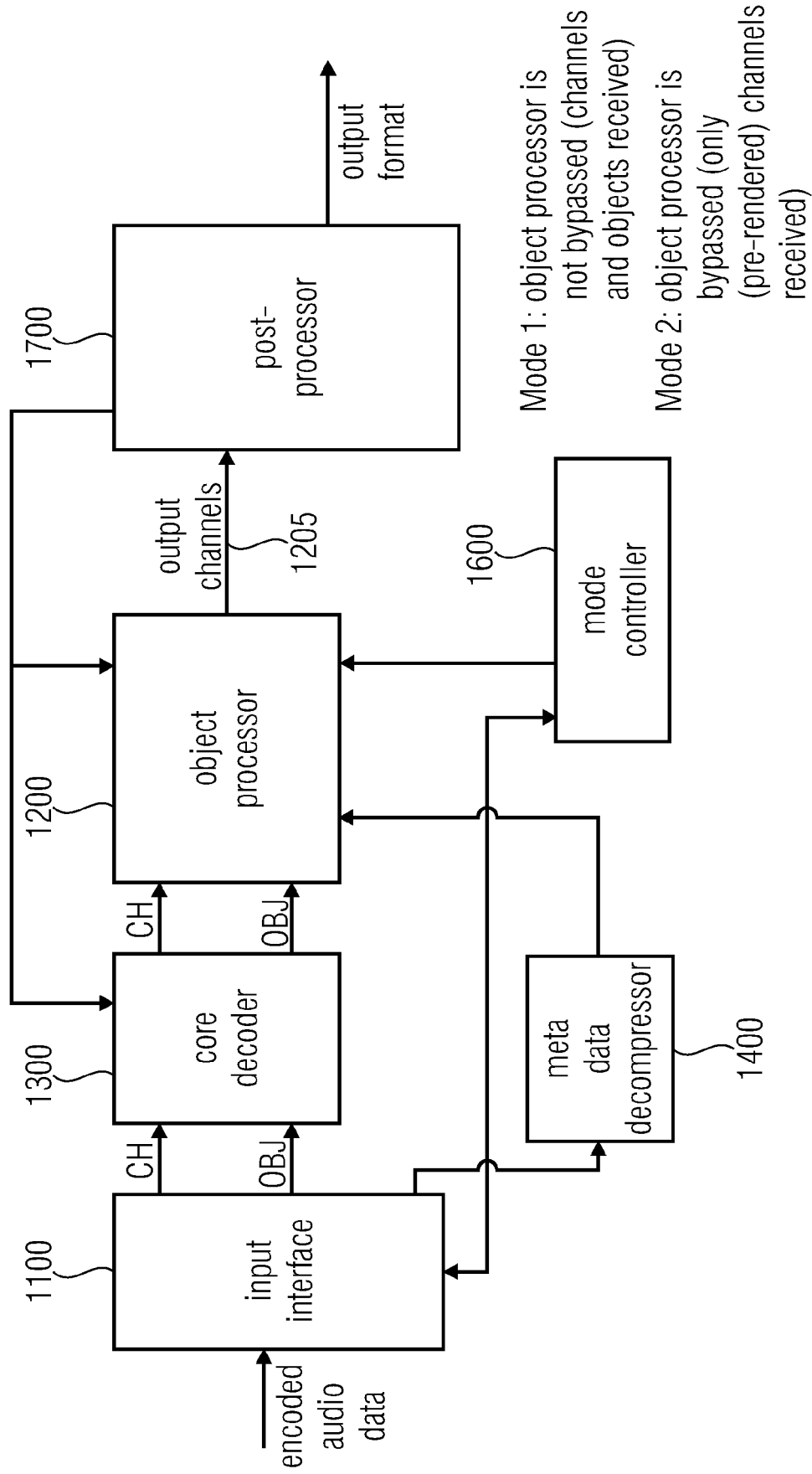
FIG 2 (DECODER)
