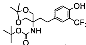
(Compound 1-1)
