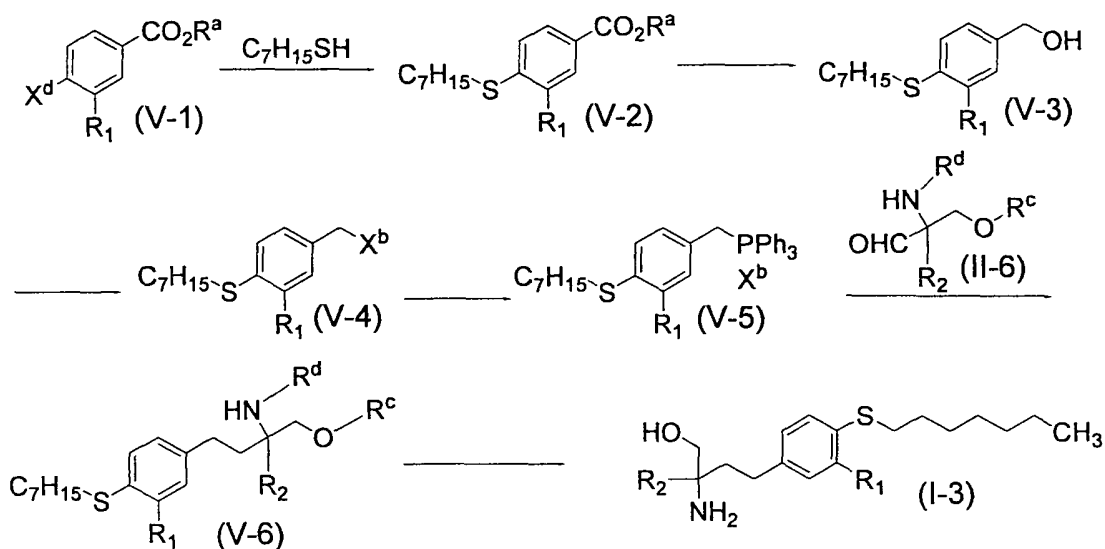
Scheme (V)
