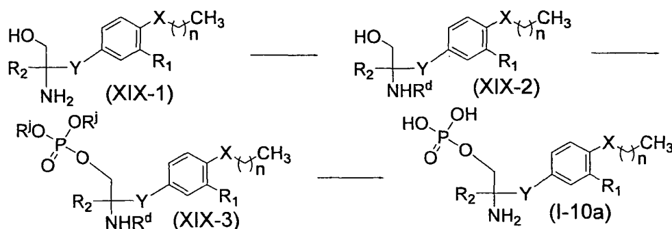
Scheme (XIX)
