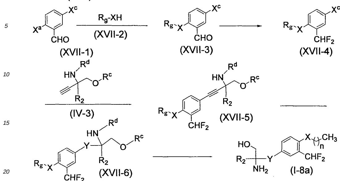
Scheme (XVII)
