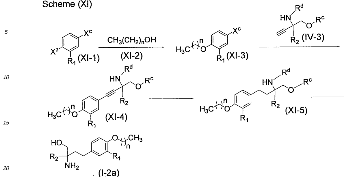
Scheme (XI)
