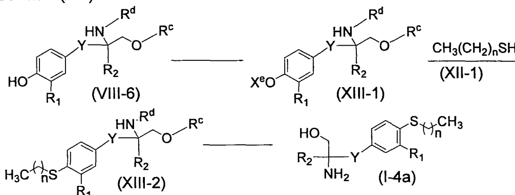
Scheme (XIII)
