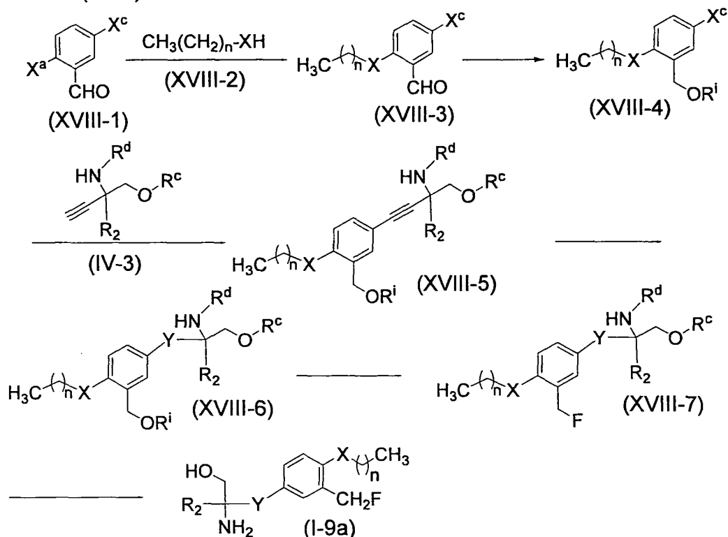
Scheme (XVIII)
