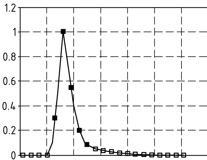
b. Symbol Rate (2/3) \times F_s , 5 significant coefficients
