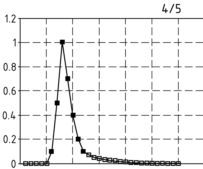
a. Symbol Rate F_s , 7 significant coefficients
