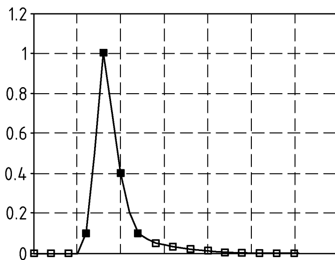
c. Symbol Rate F_s/2 , 4 significant coefficients
