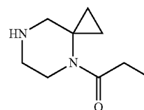
[0851] 1-(4,7-Diazaspiro[2.5]octan-4-yl)propan-1-one. LC/MS m/z 169.1 [M+H] + .
