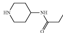
[0850] N-(Piperidin-4-yl)propionamide. LC/MS m/z 157.3 [M+H] + .
