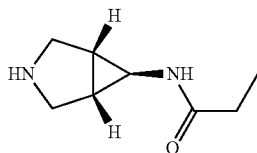
[0846] N-((1R,6S)-3-Azabicyclo[3.1.0]hexan-6-yl)propionamide. LC/MS m/z 155.3 [M+H] + .
