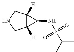
[0847] N-((1R,6S)-3-Azabicyclo[3.1.0]hexan-6-yl)propane-2-sulfonamide. LC/MS m/z 205.3
