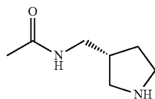
[0844] N-[(3R)-Pyrrolidin-3-yl]methyl]acetamide. LC/MS m/z 143.1 [M+H] + .
