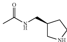
[0845] N-[(3S)-Pyrrolidin-3-yl]methyl]acetamide. LC/MS m/z 143.3 [M+H] + .
