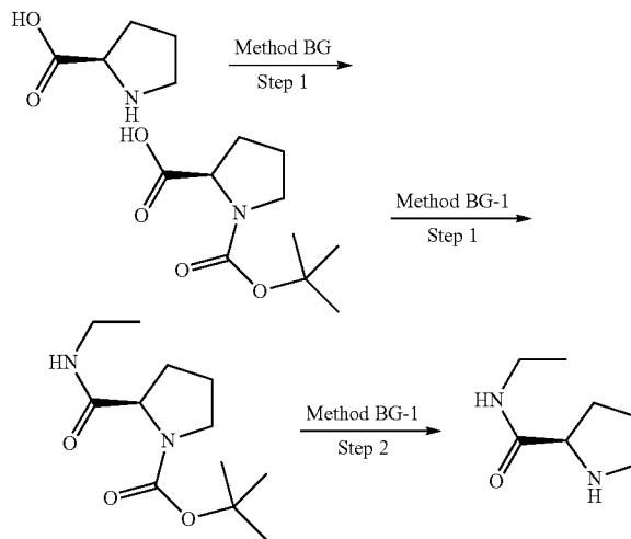
[0846] N-((1R,6S)-3-Azabicyclo[3.1.0]hexan-6-yl)propionamide. LC/MS m/z 155.3 [M+H] + .
