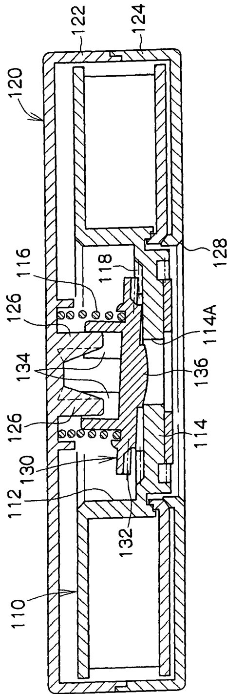
FIG.18 PRIOR ART
