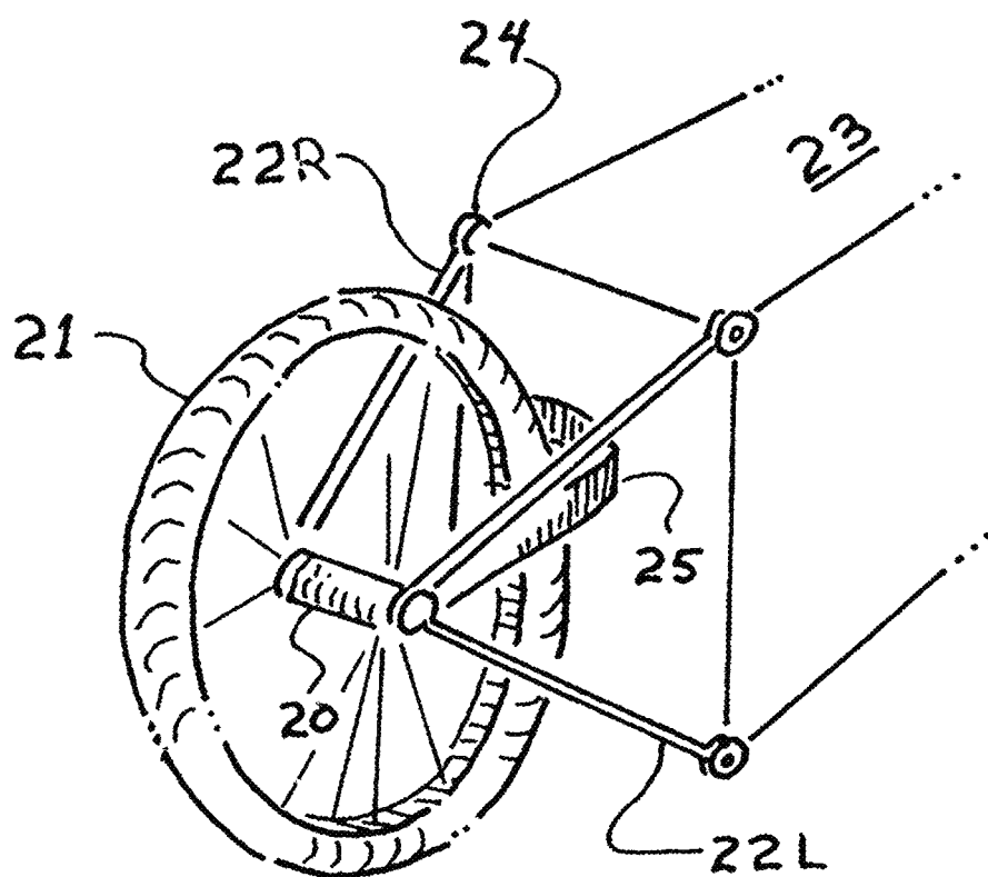
Fig. 2 (Prior Art)
