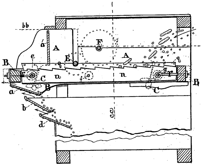
Fig. 1. Vert. Sec. on line aa fig. 4.
