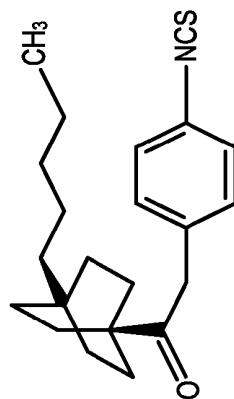
4-isothiocyanatophenyl-4-pentylbicyclo[2.2.2]octane-1-carboxylate
