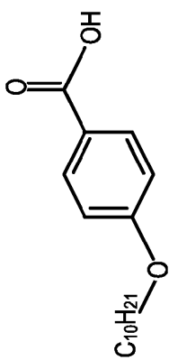
4-(decyloxy)benzoic acid
