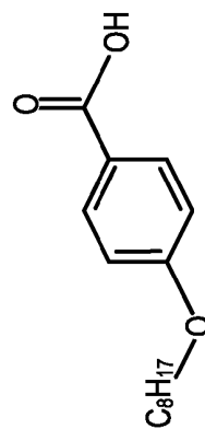
4-(octyloxy)benzoic acid
