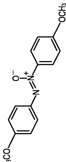
4,4'-azoxyanisole
