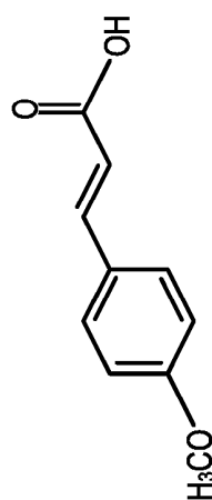
4-methoxycinnamic acid
