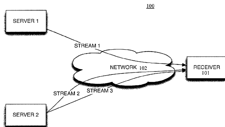
FIG. 1: System Architecture
