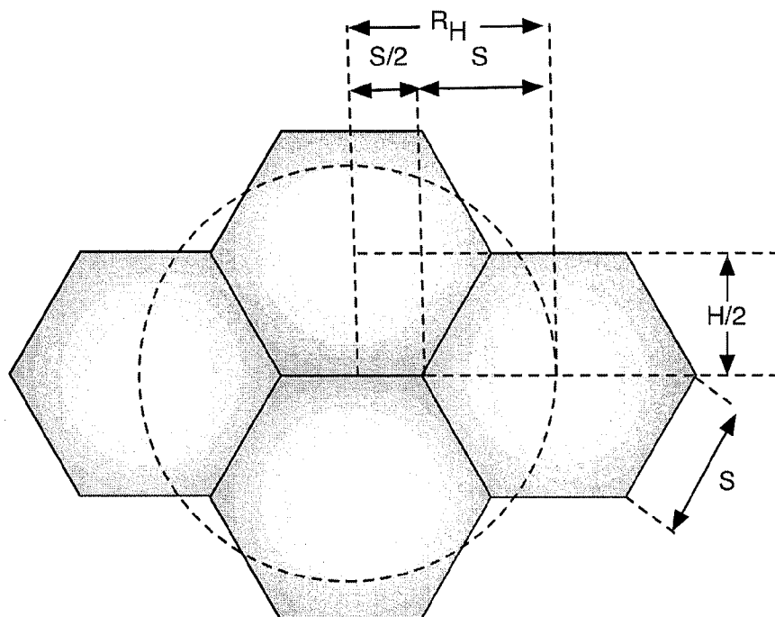
FIG. 7: View Spread of the Hexagonal Layout
