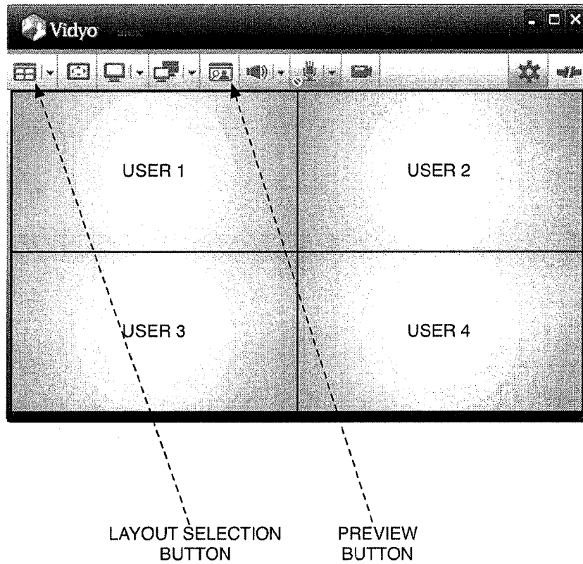
FIG. 10: User Interface - Standard Layout
