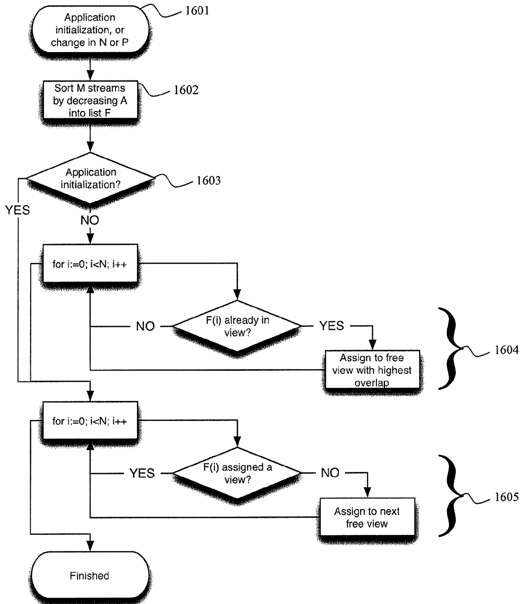
FIG. 16: Block diagram of view allocation process – layout initialization
