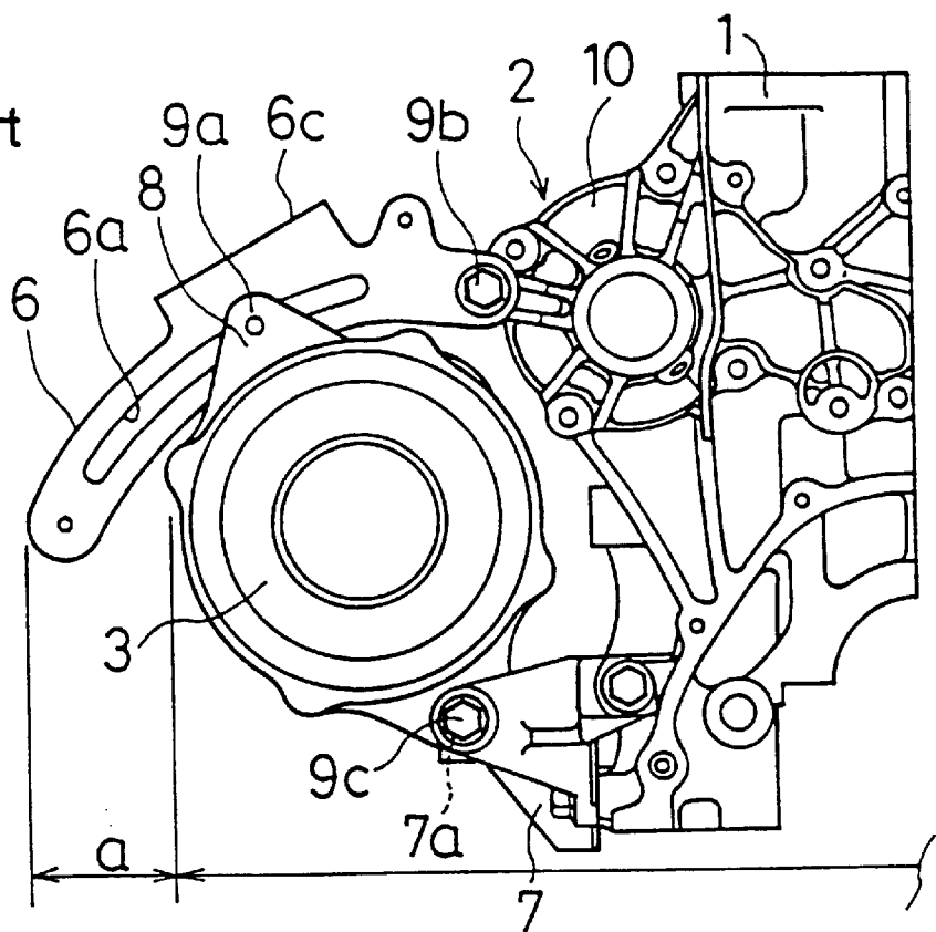
Fig. 8 Prior Art
