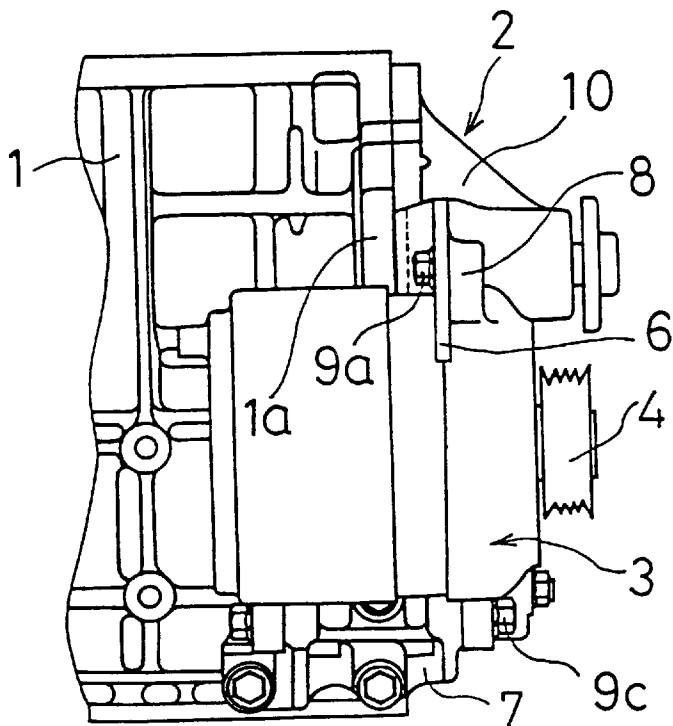
Fig. 11 Prior Art
