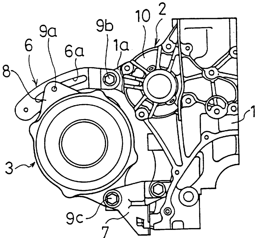
Fig. 10 Prior Art
