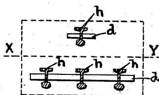
CROSS SECTION
