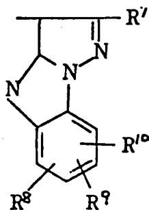
formula (11)
