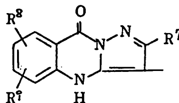
formula (12)
