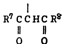
formula (15)
