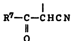
formula (14)
