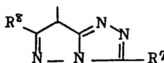
formula (10)
