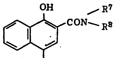
formula (8)
