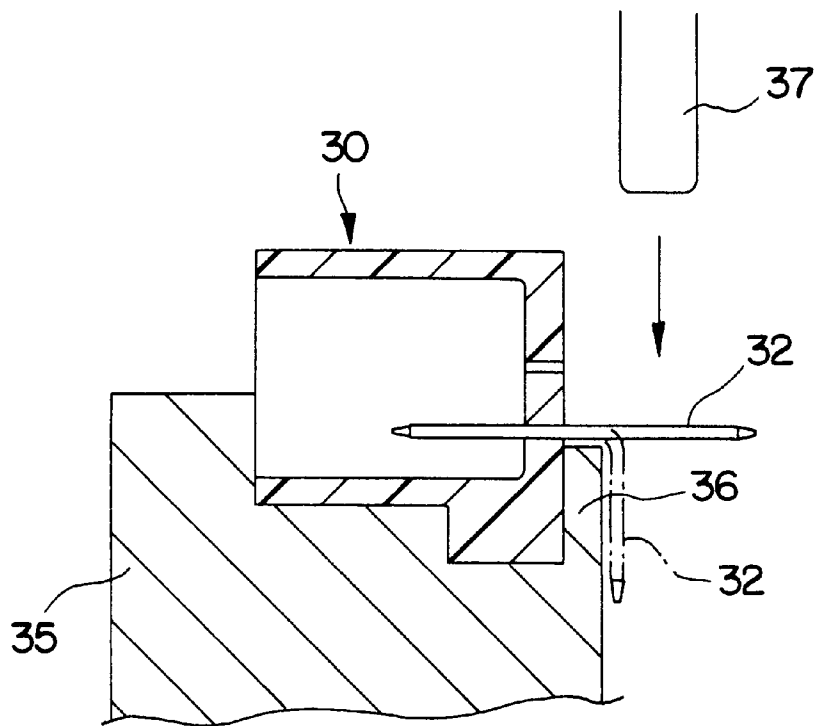
FIG. 7 PRIOR ART
