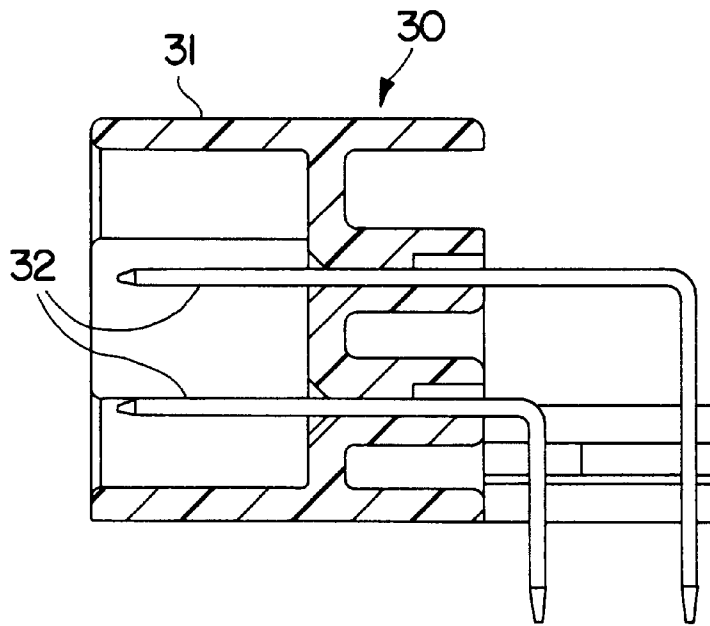
FIG. 6 PRIOR ART
