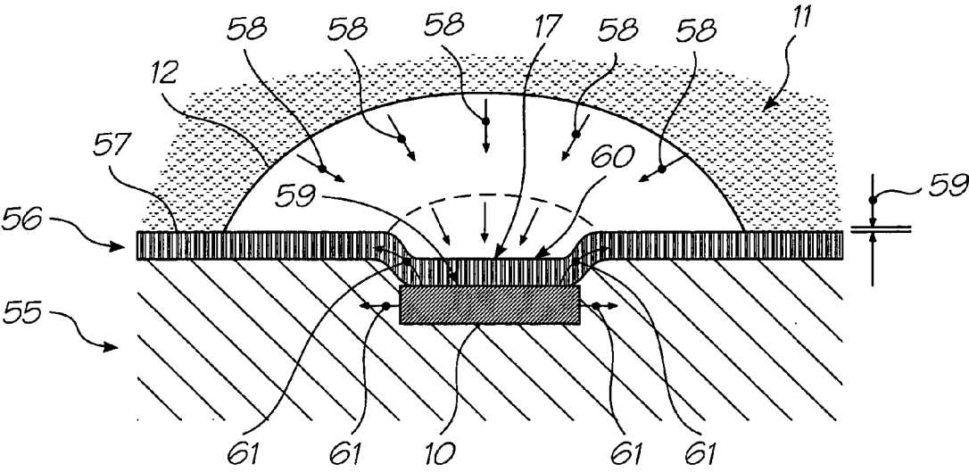
FIG. 47 (PRIOR ART)
