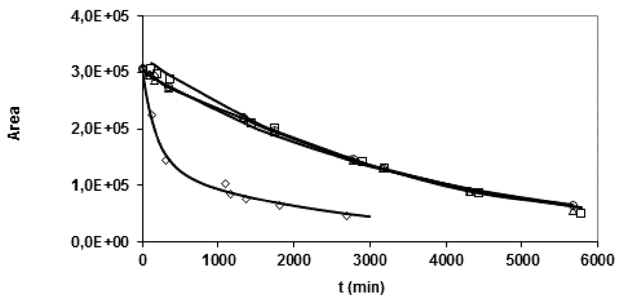
TOTAL AREA IN THE HPLC CHROMATOGRAM OF P03277 (◇) OVER TIME. AREA IN THE HPLC CHROMATOGRAM OF THE ENANTIOMERS PAIR C FUNCTIONALIZED WITH R ISOSERINOL (□), S ISOSERINOL (△) AND RACEMIC-ISOSERINOL (○) OVER TIME. THE OPEN SYMBOLS AND CURVES REPRESENT THE EXPERIMENTAL AND THE CALCULATED AREA VALUES, RESPECTIVELY. ([GdL]=0.2 mM, 1.0 M HCl, 25°C)
