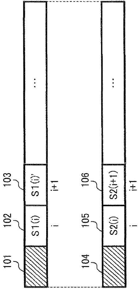
MODULATED SIGNAL A FRAME CONFIGURATION
