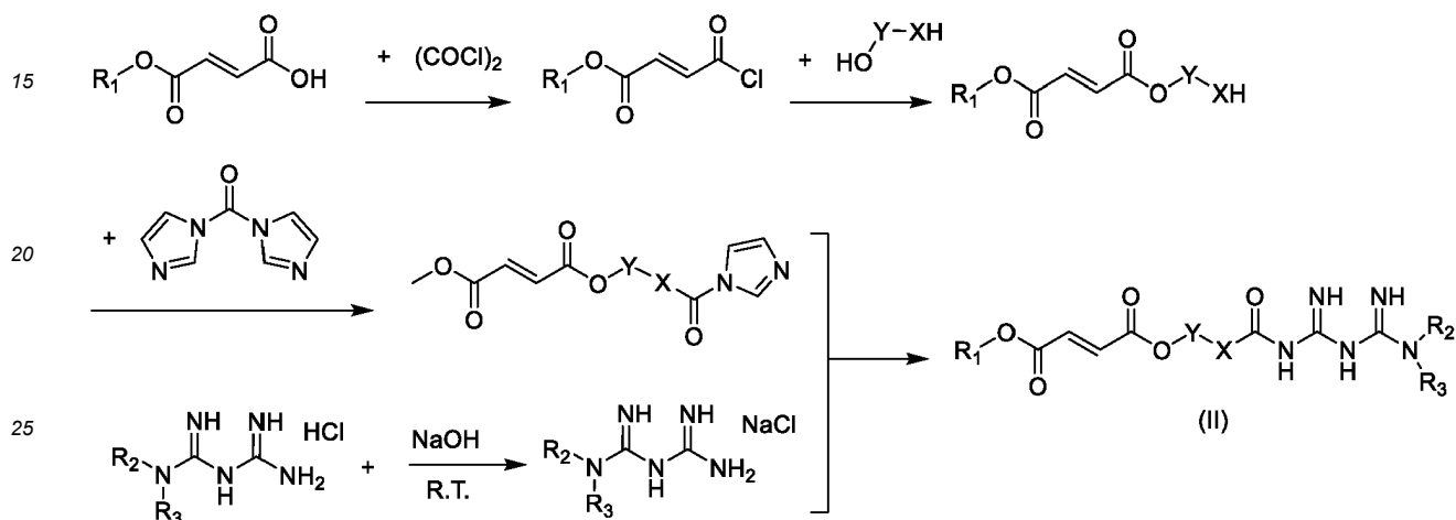
Scheme 1
