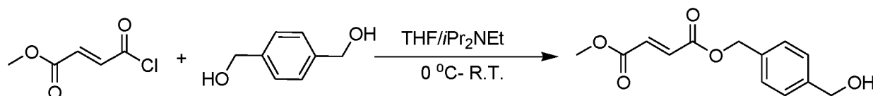
Scheme 3
