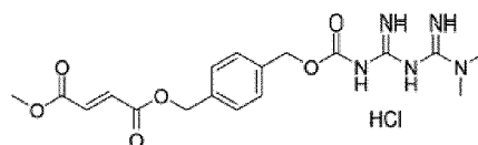
Compound 1
