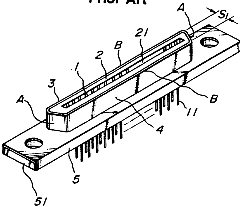
FIG. 3 Prior Art
