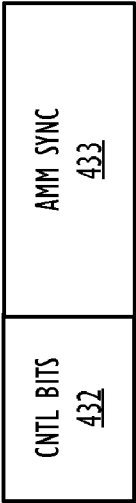
ASYNCHRONOUS MEMORY MOVE (AMM) SYNC INSTRUCTION 450
