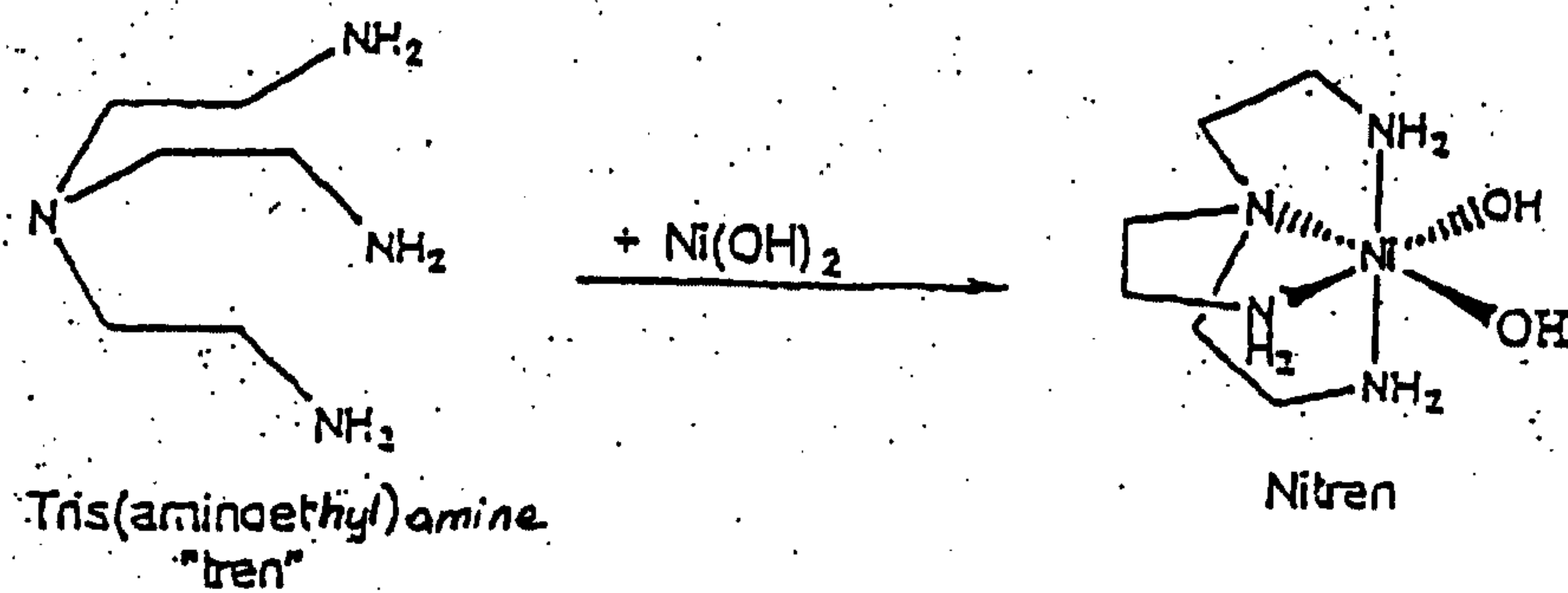
Reaction (1)
