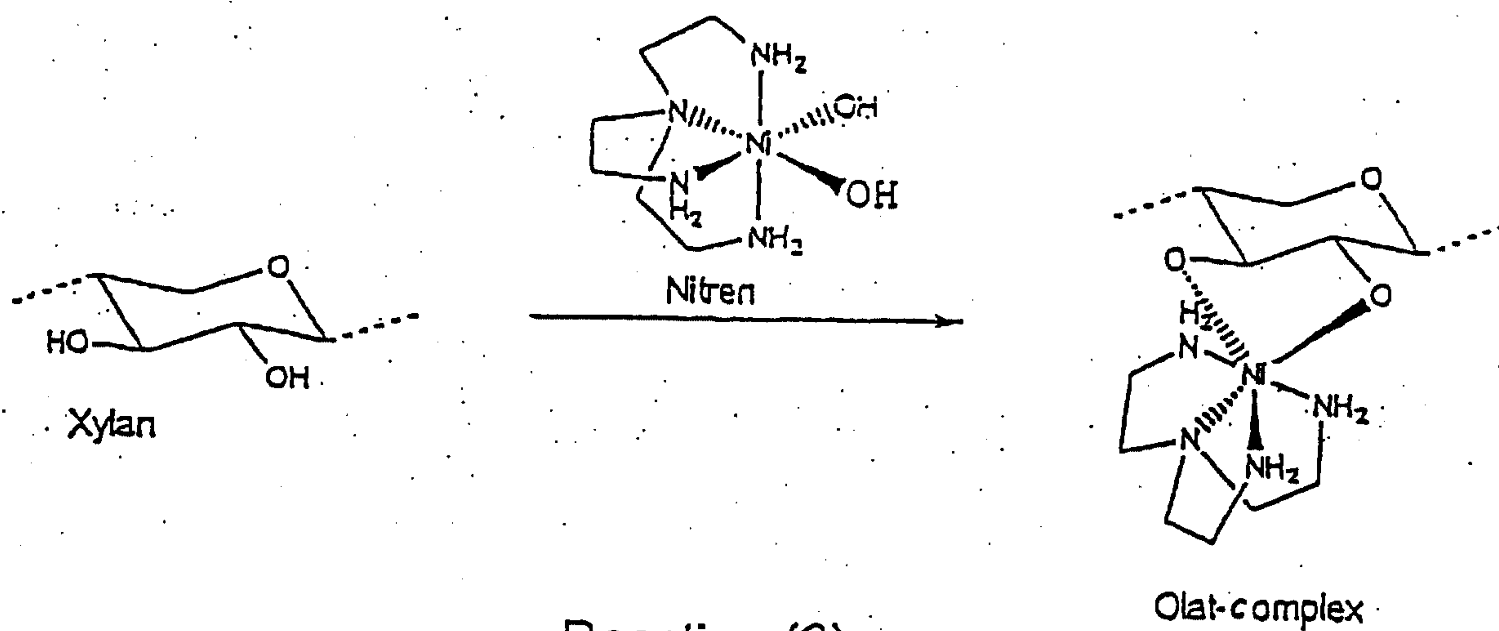
Reaction (2)
