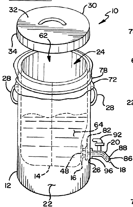
FIG. 1 PRIOR ART
