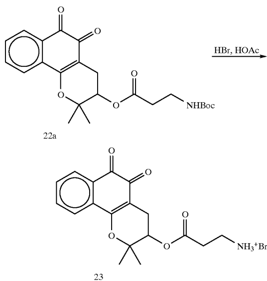
Reaction VI
