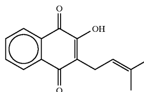
LAPACHOL
