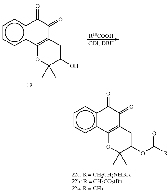
Reaction VI
