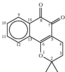
\beta -LAPACHONE
