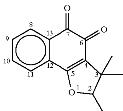
\beta -LAPACHONE
