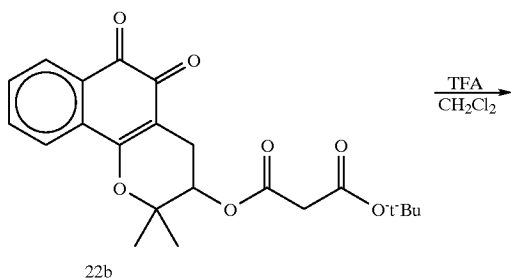
Reaction VII
