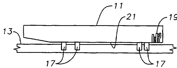
Fig. 2 (Prior Art)
