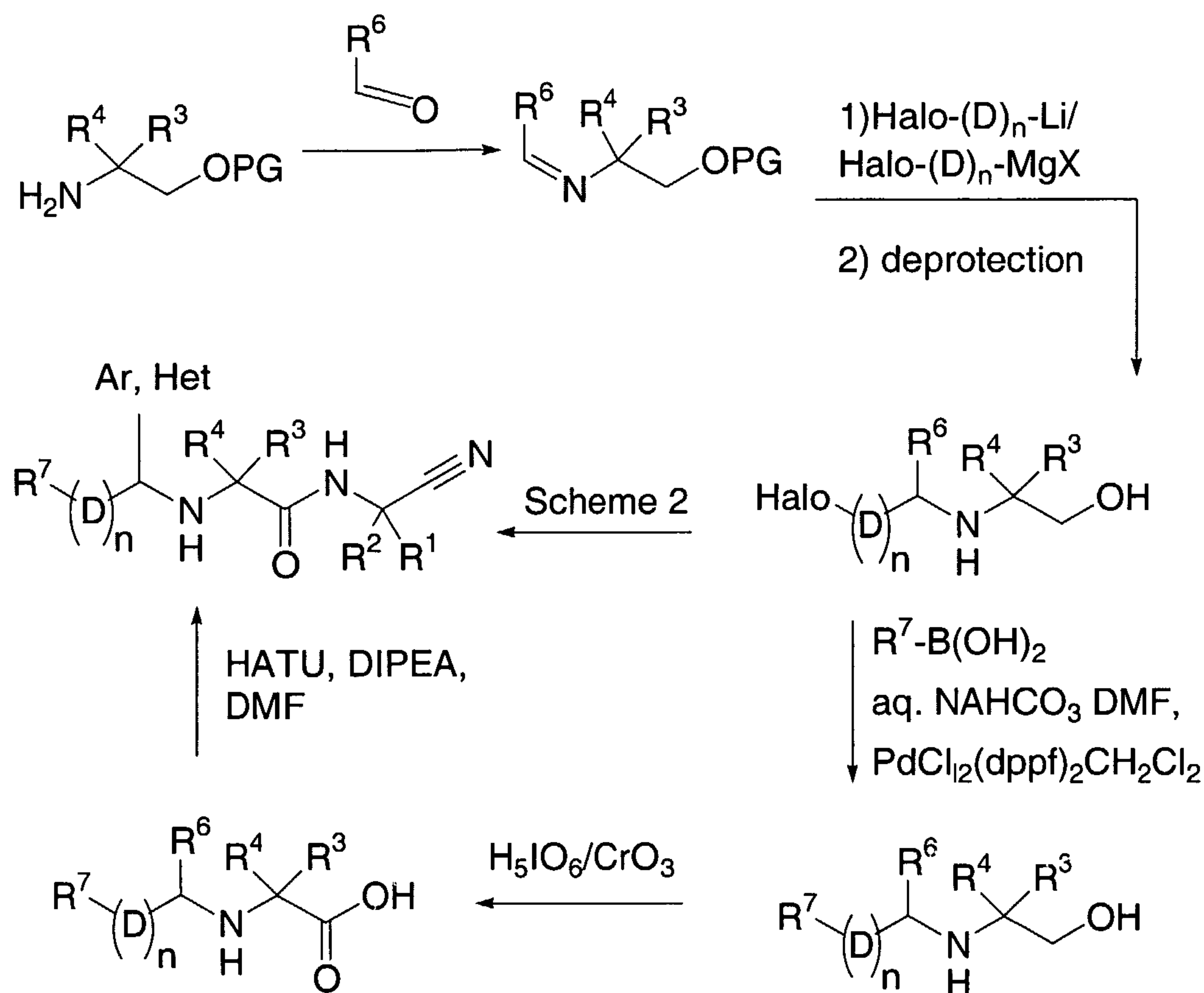
SCHEME 12
