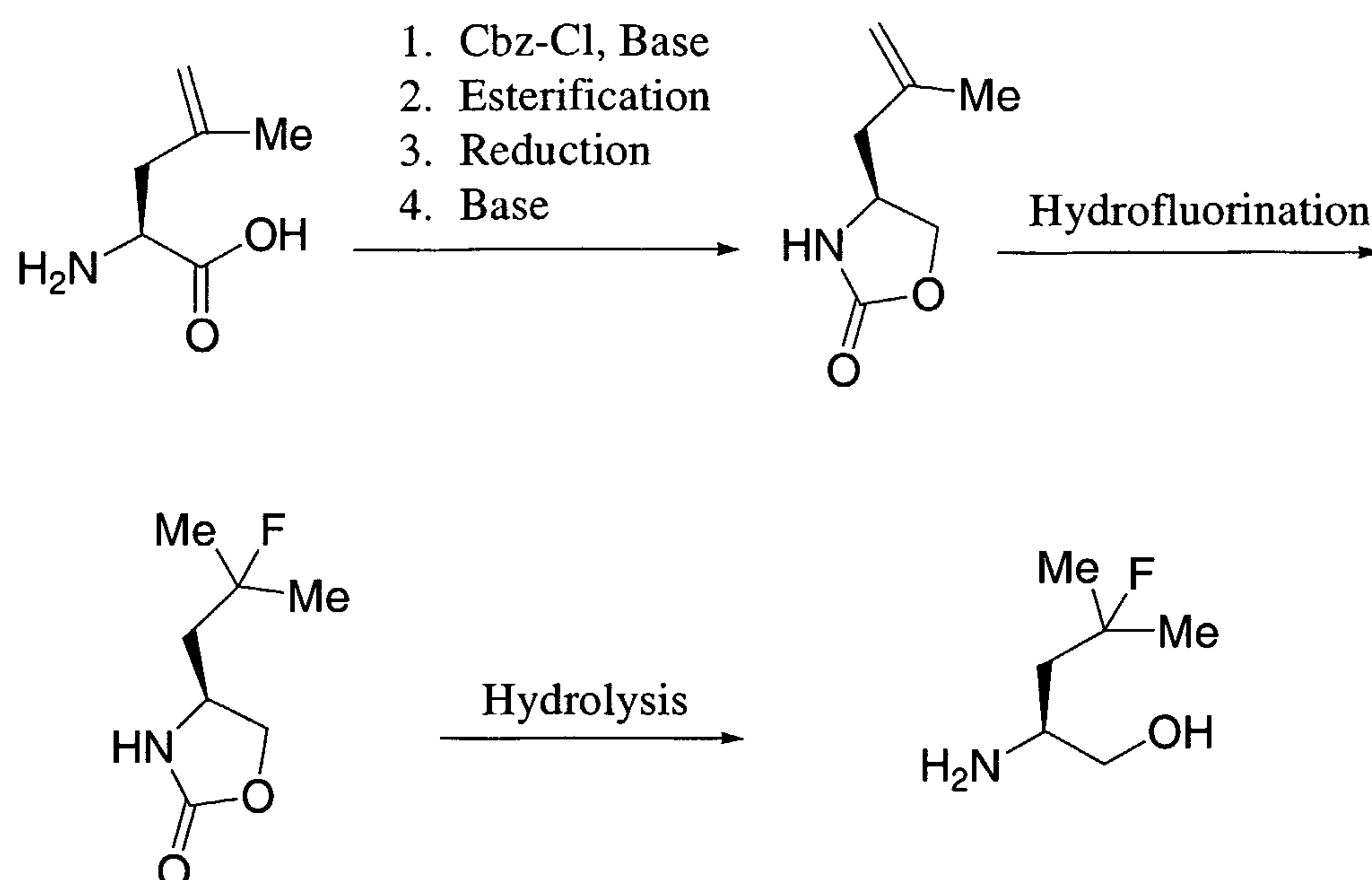
SCHEME 8
