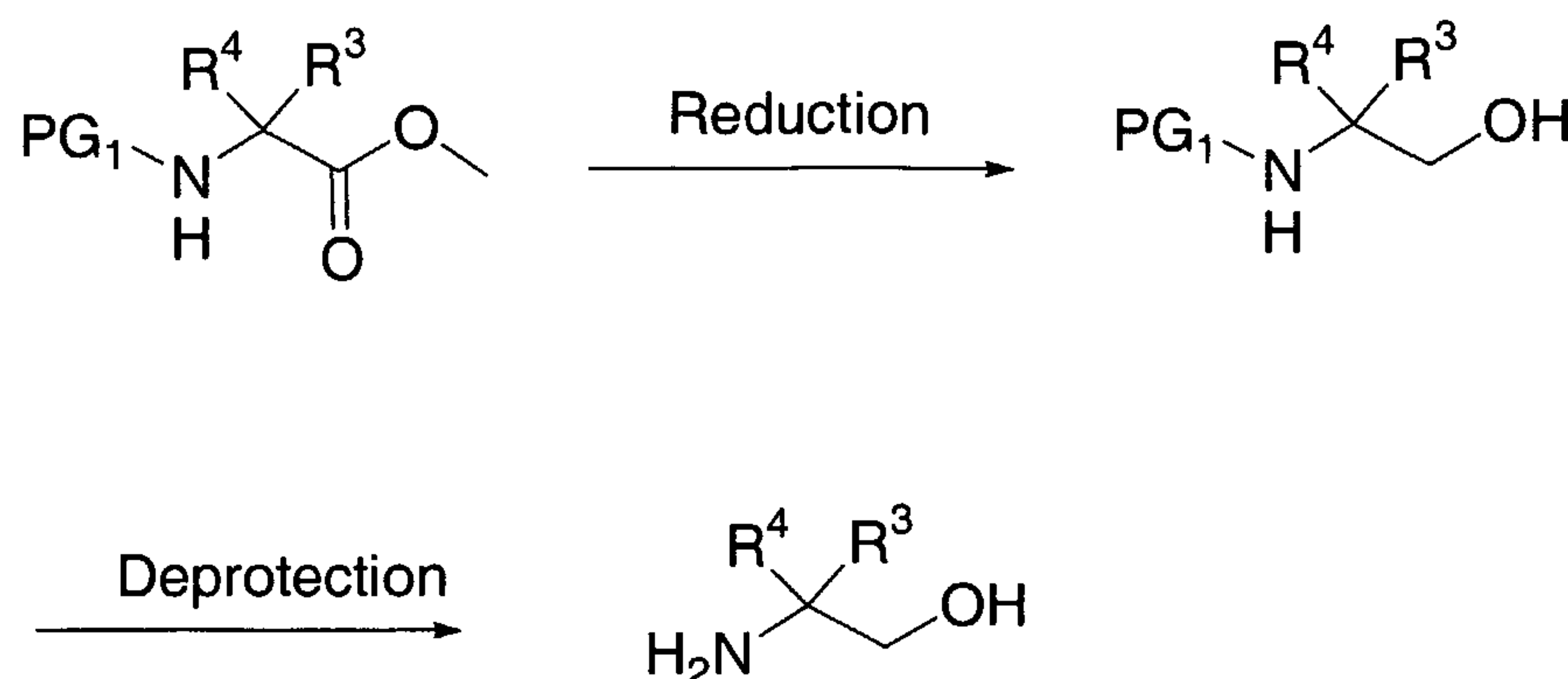
SCHEME 10
