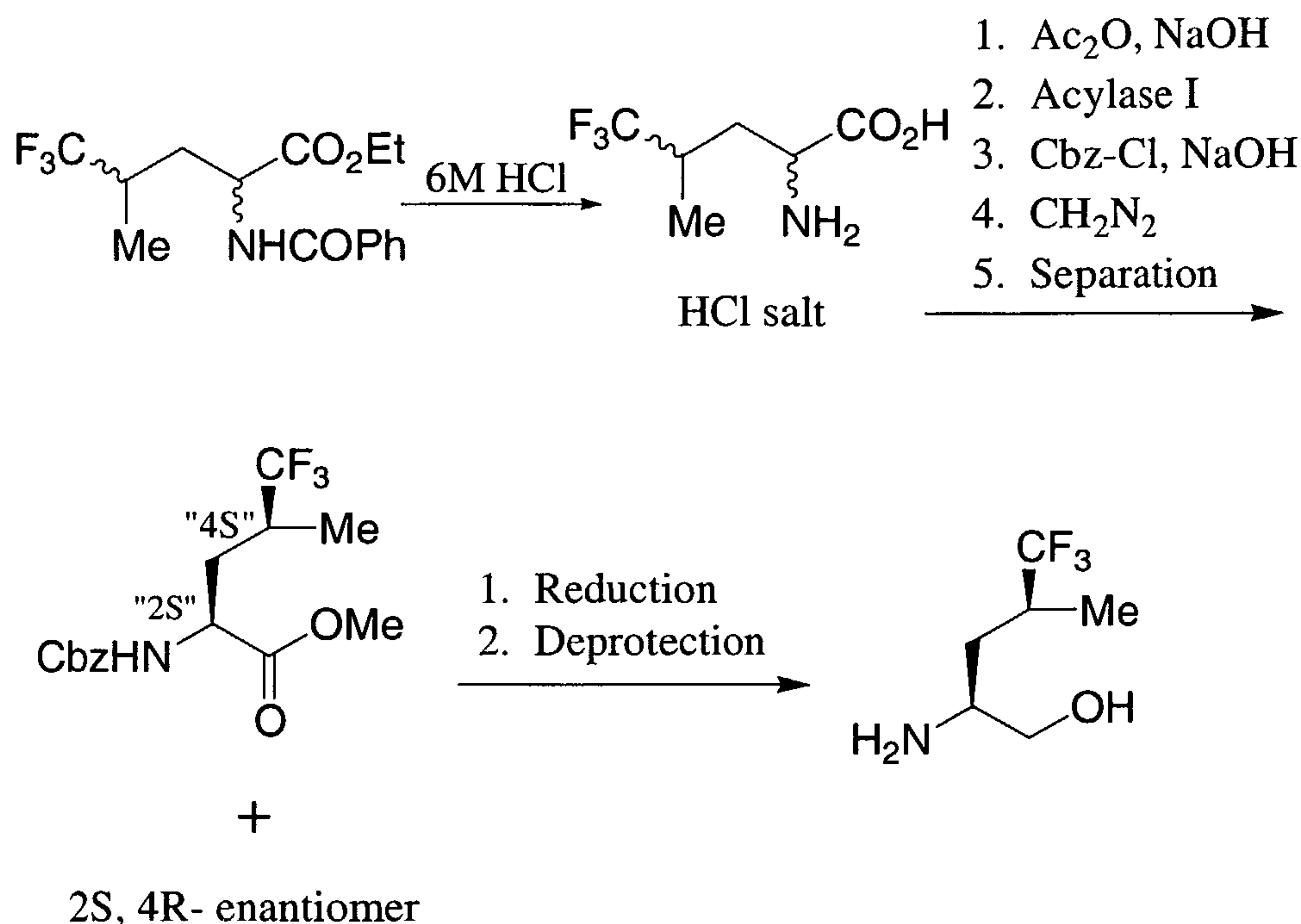
SCHEME 11
