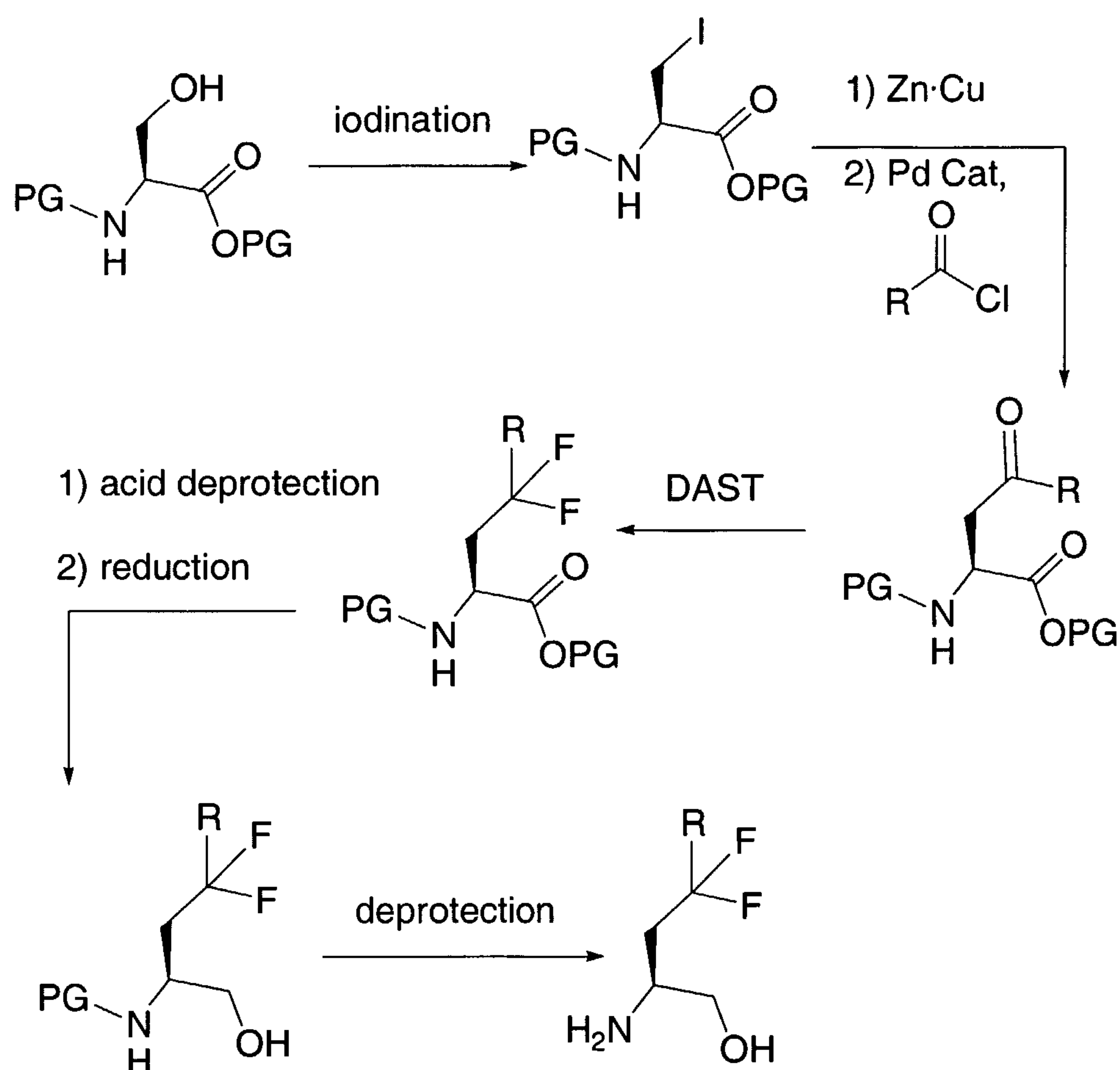
SCHEME 9
