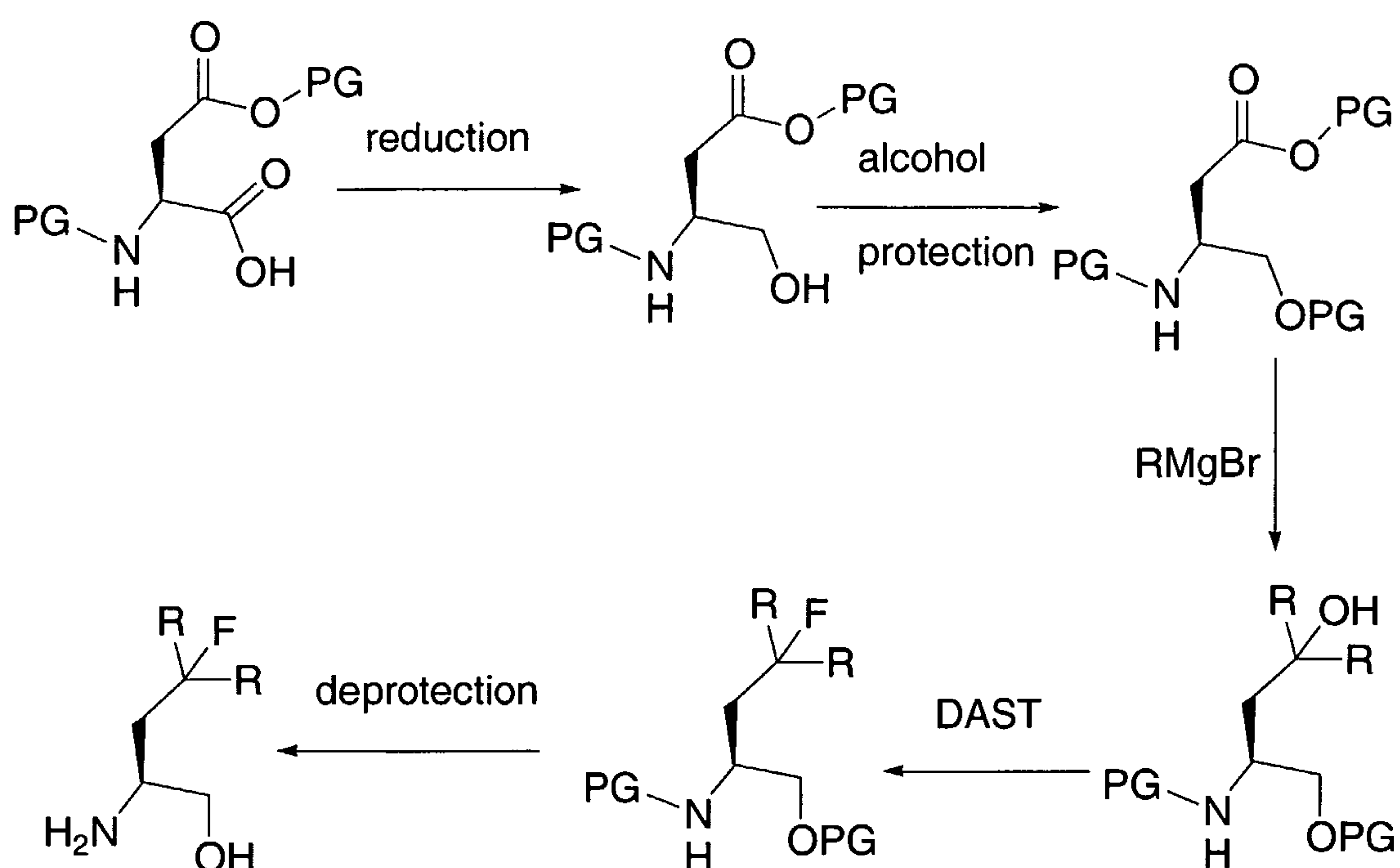
SCHEME 7
