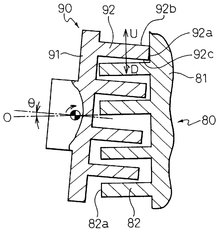
Fig. 11 (PRIOR ART)
