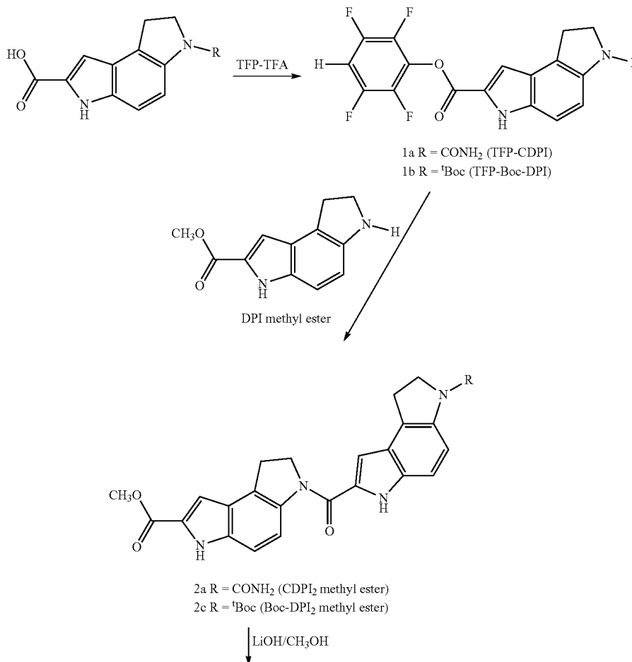
Reaction Scheme 1
