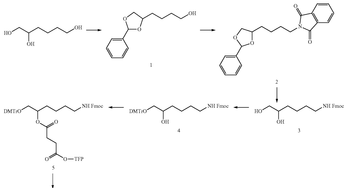
Scheme 6: Preparation of CDPI 3 —CPG support (below)
