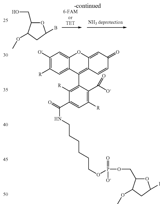
Scheme 8: Introduction of fluorophores at the 5'-end using 6-FAM and TET phosphoramidites (below)
