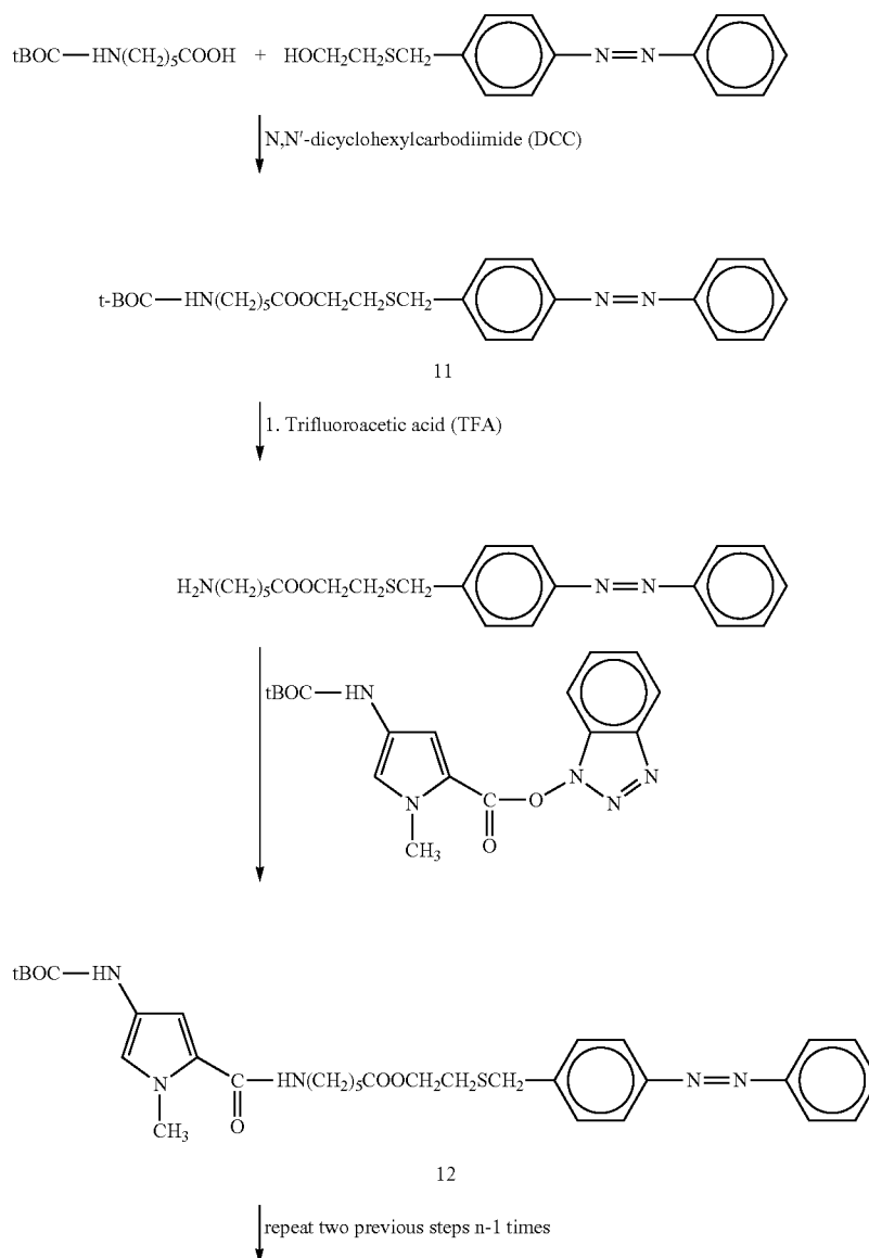
Reaction Scheme 2
