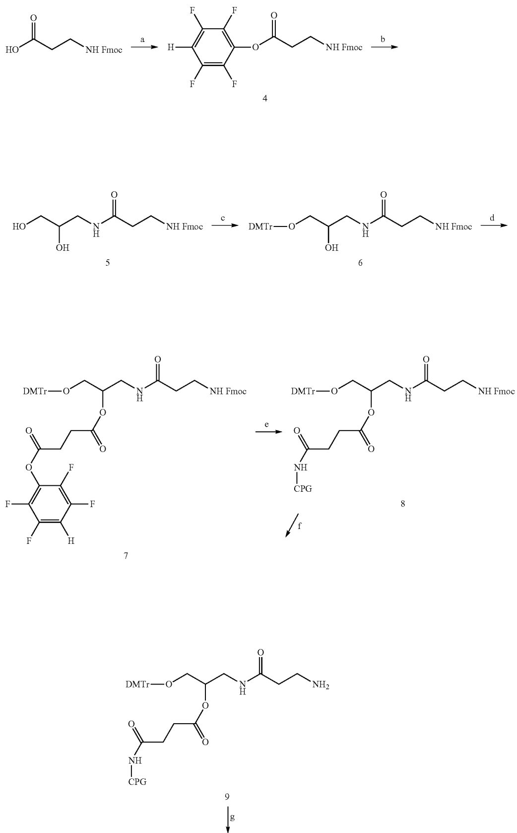
Reaction Scheme 5
