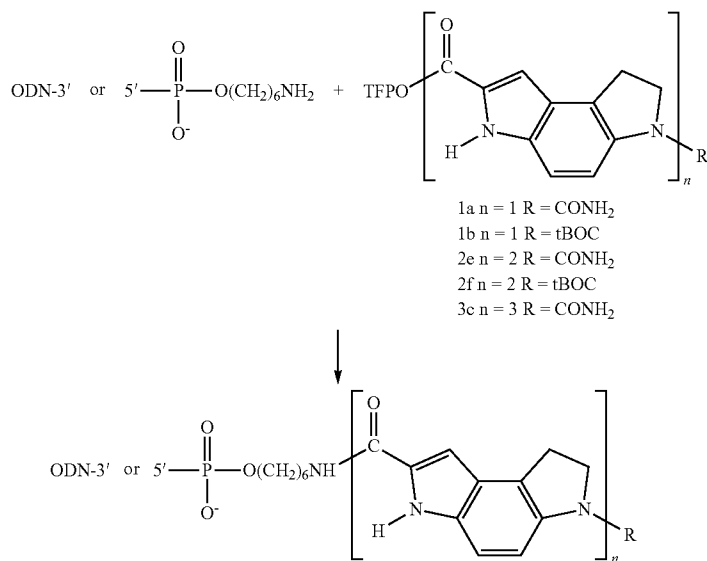
Reaction Scheme 3
