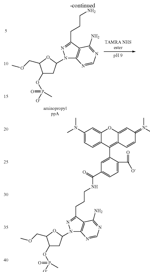
Scheme 9: Postsynthesis introduction of TAMRA quencher at the internal ppG or ppA residues (below)
