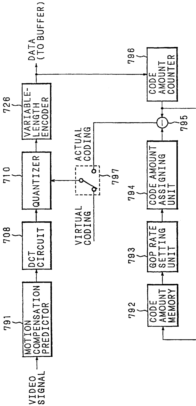
FIG. 14 PRIOR ART
