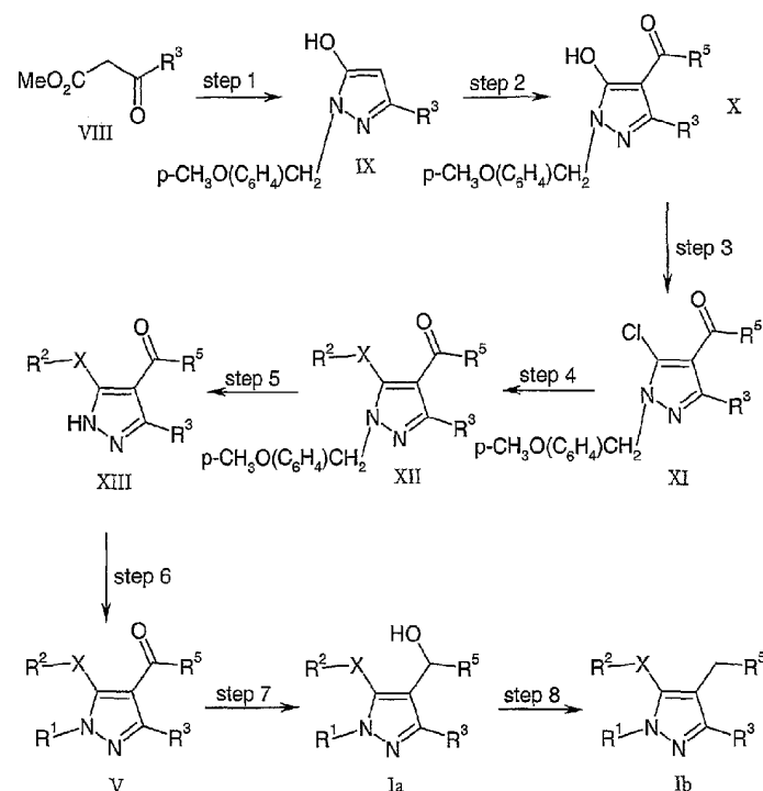
Reaction scheme 3:
