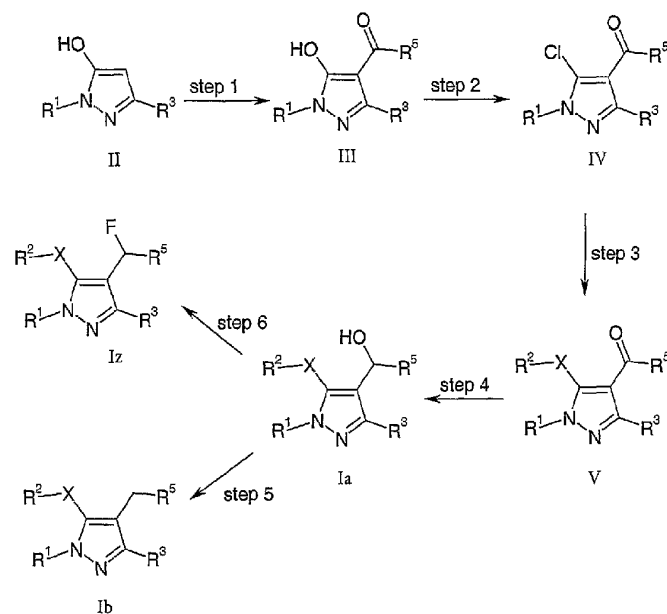
Reaction scheme 1:
