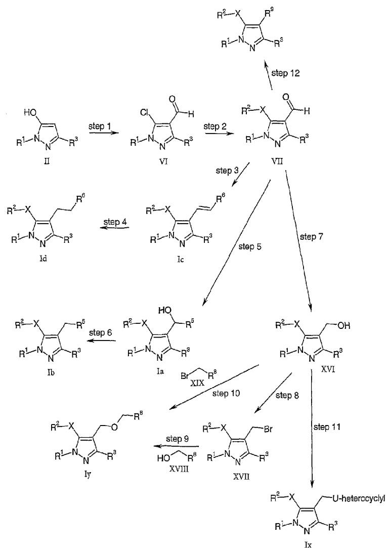
Reaction scheme 2:
