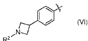
[Chemical Formula 15]
