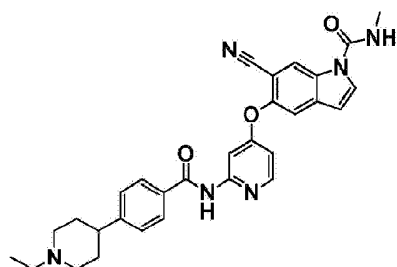
[Chemical Formula 178]
