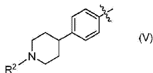
[Chemical Formula 15]
