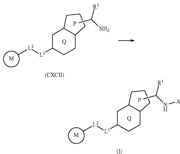
&lt;Reaction Scheme 27&gt;
