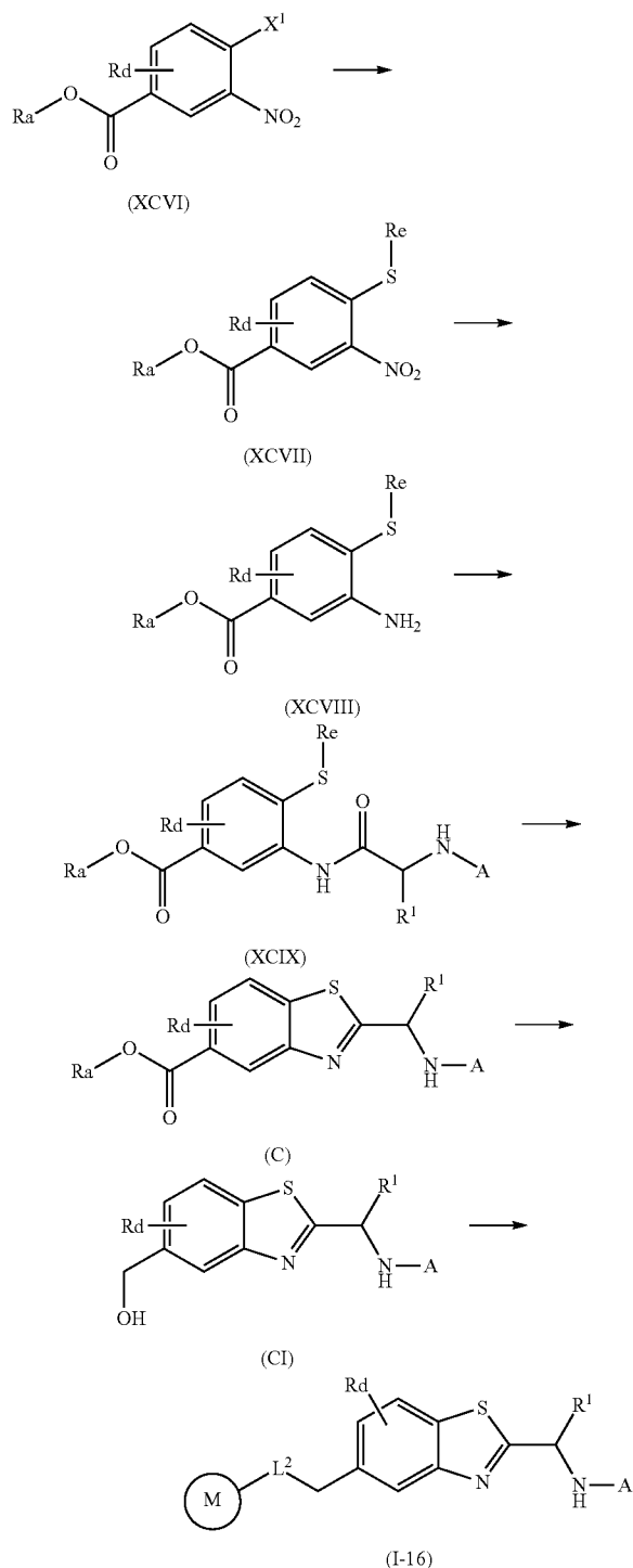
&lt;Reaction Scheme 16&gt;
