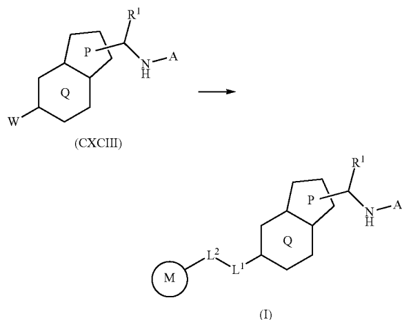
&lt;Reaction Scheme 28&gt;
