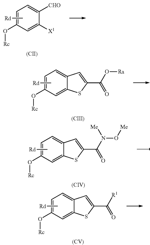
&lt;Reaction Scheme 17&gt;
