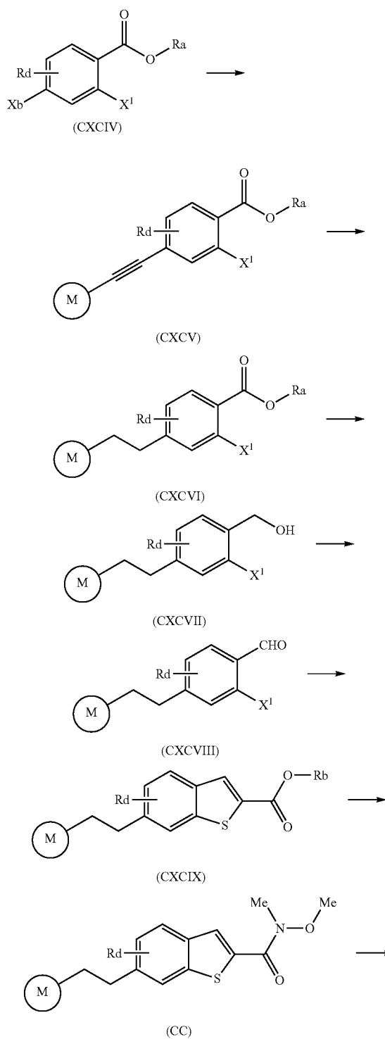
&lt;Reaction Scheme 29&gt;
