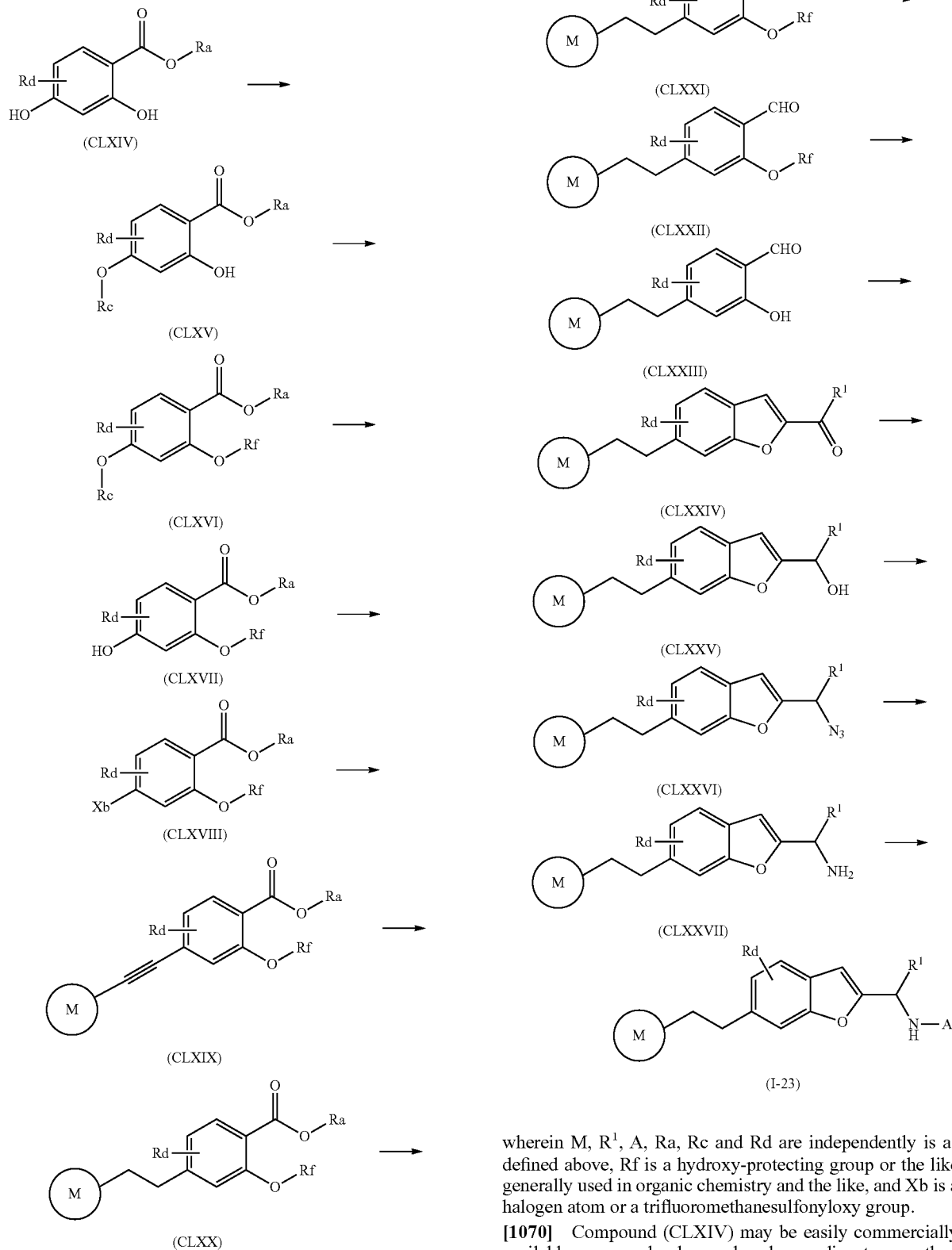
&lt;Reaction Scheme 25&gt;
