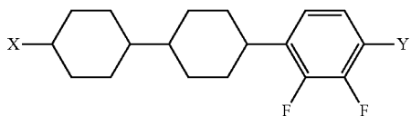
Chemical Formula 11
