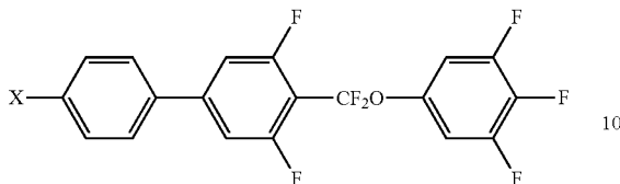
Chemical Formula 16 5
