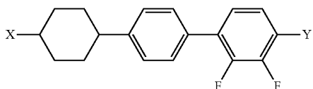
Chemical Formula 12
