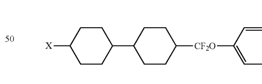
Chemical Formula 4
