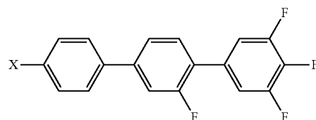
Chemical Formula 12
