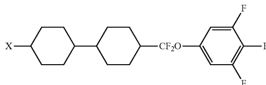
Chemical Formula 4
