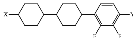
Chemical Formula 10
