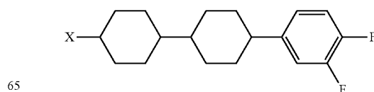
Chemical Formula 5
