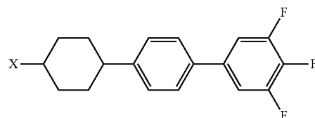
Chemical Formula 11
