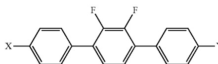
Chemical Formula 10
