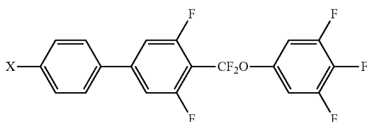
Chemical Formula 6 10
