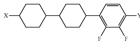
Chemical Formula 9
