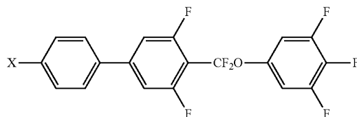
Chemical Formula 6
