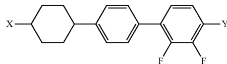
Chemical Formula 4 40
