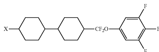
Chemical Formula 14 30
