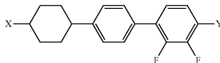
Chemical Formula 12 40
