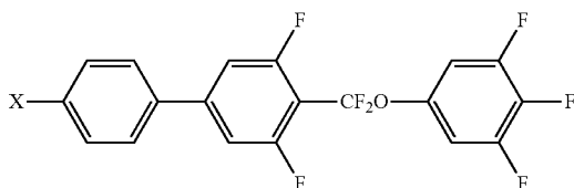
Chemical Formula 16
