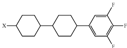
Chemical Formula 17
