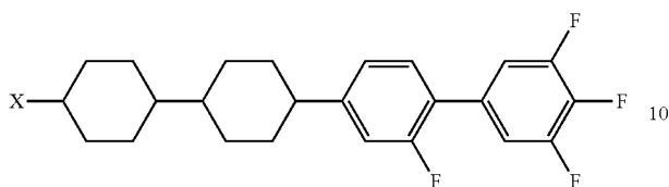
Chemical Formula 8
