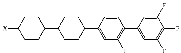
Chemical Formula 18
