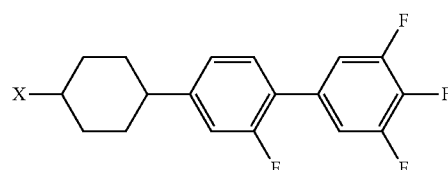
Chemical Formula 13 20
