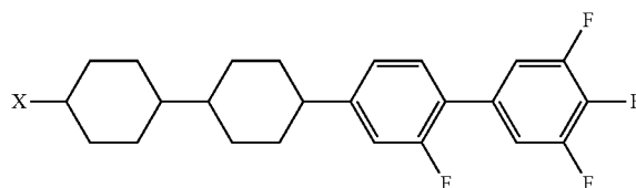
Chemical Formula 8
