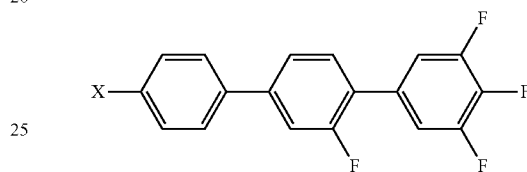
Chemical Formula 2
