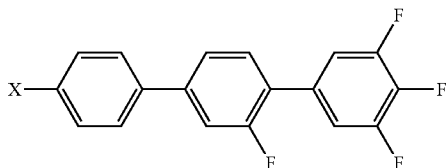
Chemical Formula 2
