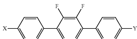
Chemical Formula 10 45
