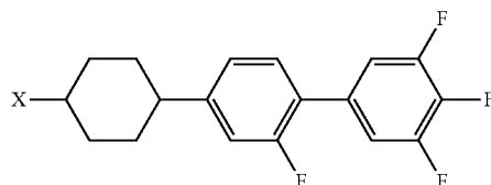
Chemical Formula 3
