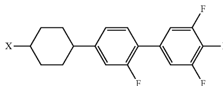
Chemical Formula 13
