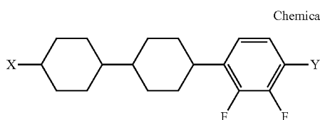
Chemical Formula 9 35
