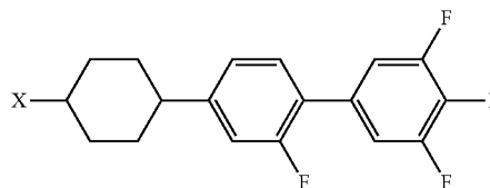
Chemical Formula 3
