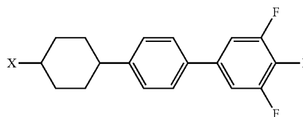
Chemical Formula 11
