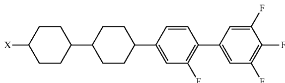
Chemical Formula 18
