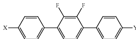
Chemical Formula 13 45
