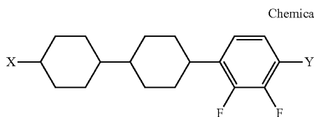
Chemical Formula 9
