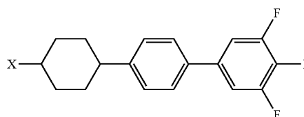
Chemical Formula 1
