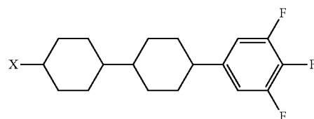
Chemical Formula 8
