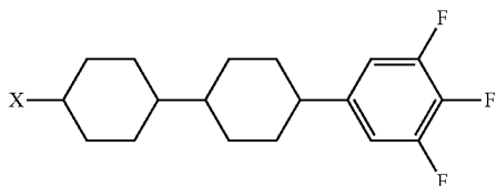
Chemical Formula 17 5
