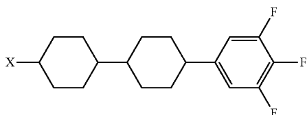
Chemical Formula 17
