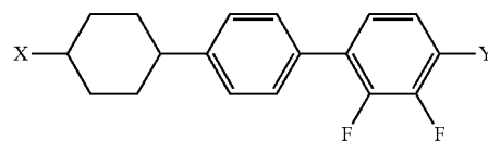
Chemical Formula 11
