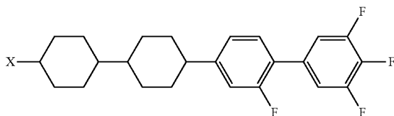
Chemical Formula 18
