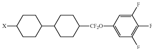
Chemical Formula 14
