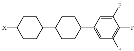
Chemical Formula 7 15
