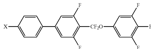
Chemical Formula 16 55
