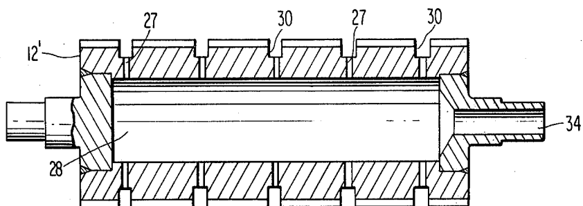
FIG 5 PRIOR ART
