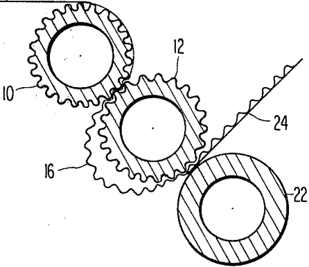
FIG 3 PRIOR ART
