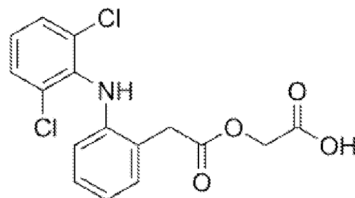
aceclofenac
