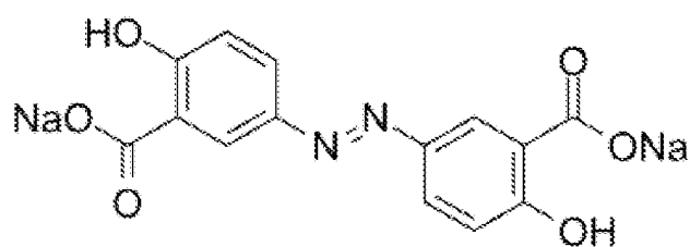
olsalazine
