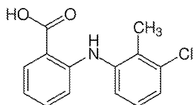
tolfenamic acid
