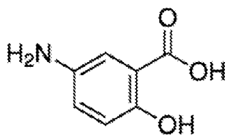
5-aminosalicylic acid
