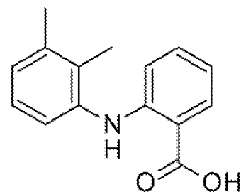
mefenamic acid
