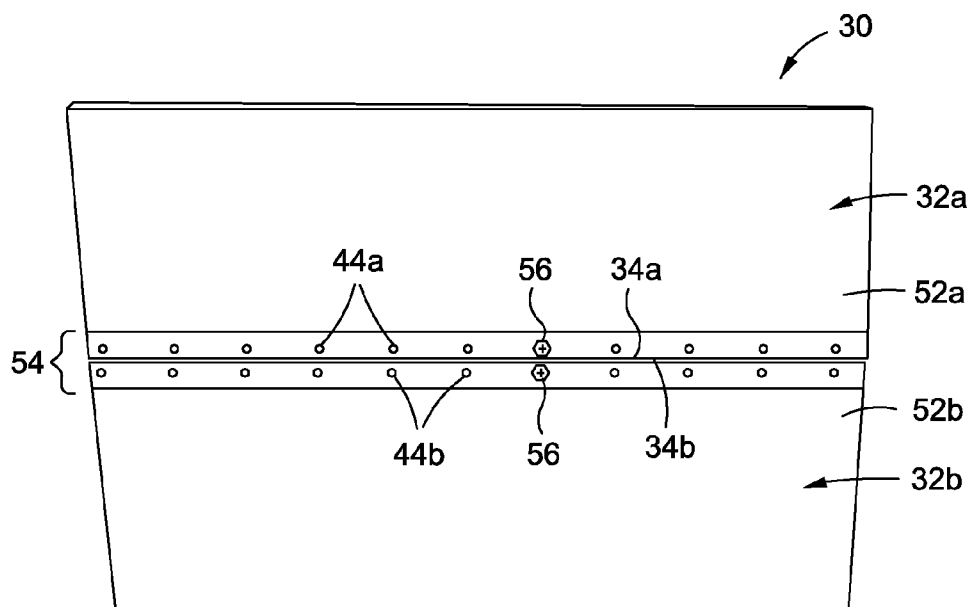
FIG. 2C (PRIOR ART)
