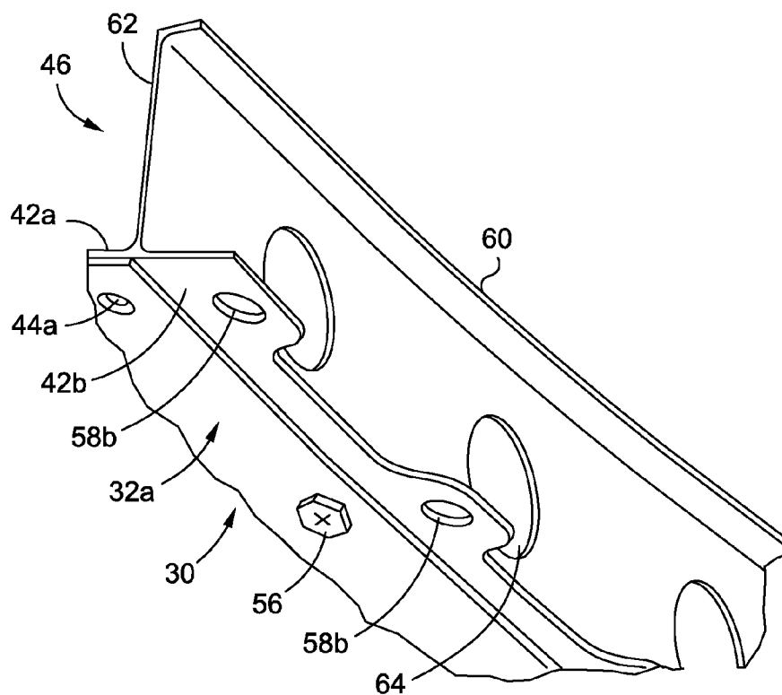
FIG. 3 (PRIOR ART)
