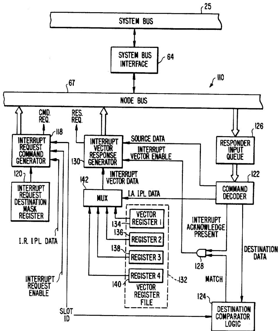
FIG. 6. INTERRUPTING NODE
