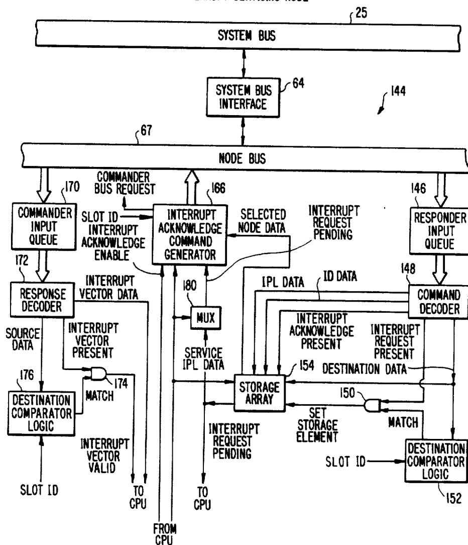
FIG. 7 INTERRUPT SERVICING NODE
