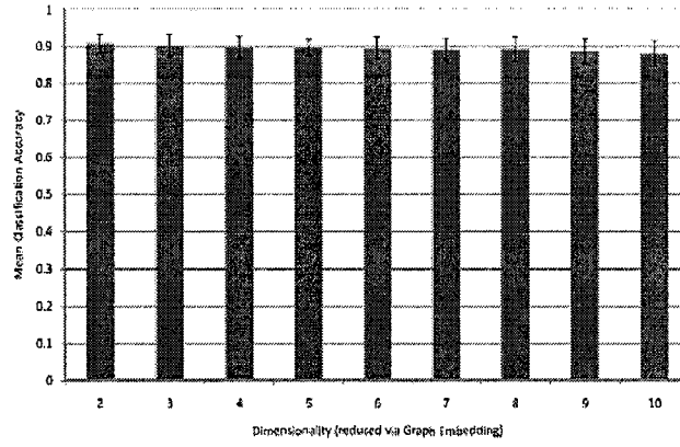
Fig. 12. The mean ( \mu_{ACC} ) classification accuracy over 100 trials of 3-fold cross-validation is shown for different dimensionalities \{2, 3, \dots, 10\} obtained via Graph Embedding. The error bars represent standard deviation ( \sigma_{ACC} ) of the classification accuracy.
