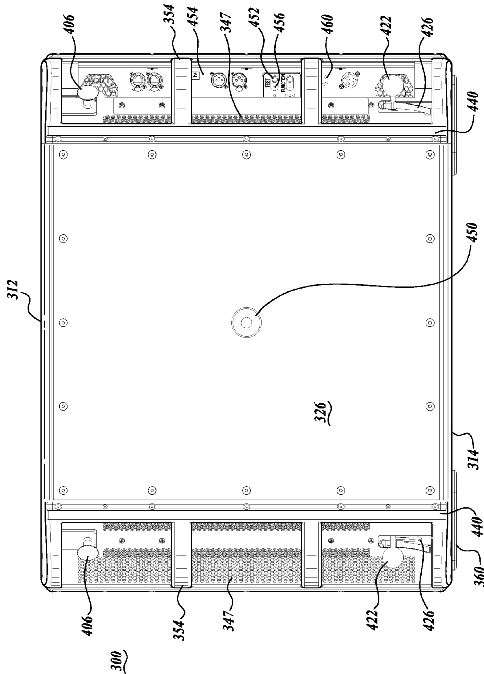
Fig. 38. (FRONT VIEW)
